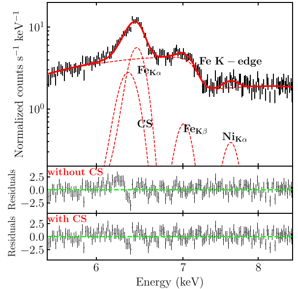
Figure 1. A representative spectrum of GX 301-2 in our sample (ObsID:P010130901601; upper panel). The spectrum is fitted in the energy range of 5.5–8.5 keV with an absorbed ( tbabs ) powerlaw model including three emission lines, i.e. Fe K \alpha , Fe K \beta , and Ni K \alpha and an additional CS described as a box function. We show residuals with and without the CS component in the two bottom panels.
