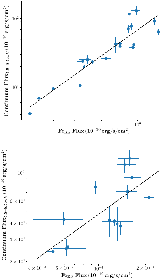
Figure 4. The upper (lower) panel shows the relation between the Fe K\alpha (Fe K\beta ) flux and the unabsorbed flux of the continuum in the energy range of 5.5–8.5 keV. Dashed lines represent linear fits in the logarithmic space, which result in linear coefficients of 1.25 and 0.88 for Fe K\alpha and Fe K\beta lines, respectively.
