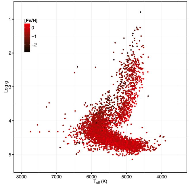
Figure 2. Location of our sample, consisting of 4675 stars, in the H-R diagram. The stars are colour coded according to their measured [\text{Fe}/\text{H}] .
