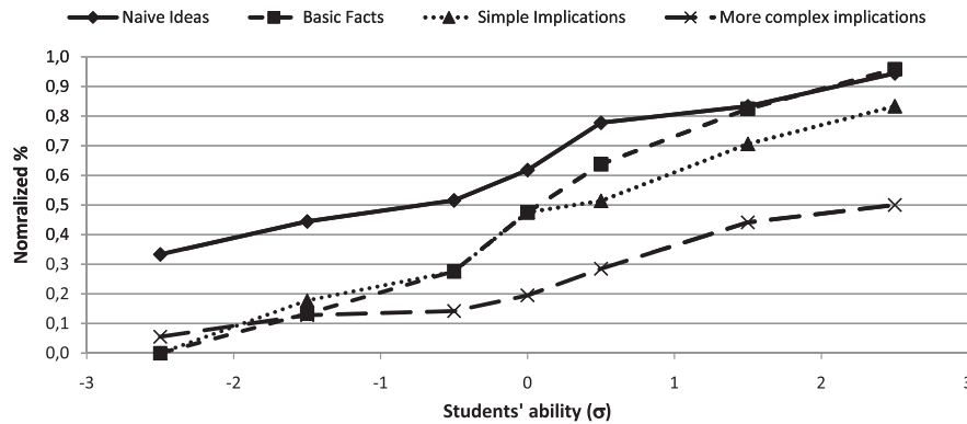
FIG. 7. IRC for cluster levels of the learning progression about change of seasons, Moon phases, and solar or lunar eclipses.
