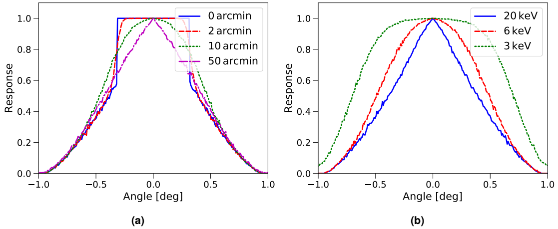
Figure 17: Effect on the response of a collimator by inner-wall grazing reflection of photons, as simulated through the Monte Carlo algorithm explained in the text. a) Fixed energy (6.4 keV), variable roughness (expressed in arcmin). The step-like response due to the grazing reflection at 0 arcmin happens between \pm\alpha_C . Roughness acts like a gaussian smoothing on the step. b) Fixed roughness (6 arcmin), variable energy.
