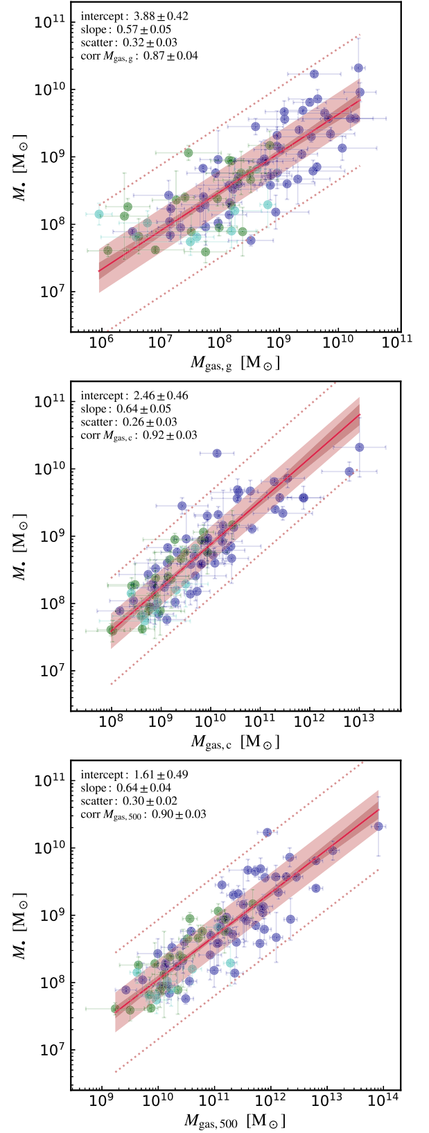
Figure 6. Black hole mass vs. enclosed gas mass (Section 3.2.3) within R_{x,g} (top), R_{x,c} (middle), and R_{500} (bottom). Although M_{\text{gas}} is a derived property, M_{\bullet}-M_{\text{gas}} is tight across all regions, and shows a nearly maximal positive correlation coefficient in the core region. Compared with the stellar mass (Magorrian) relation, the scatter is halved and is analogous to the fundamental T_x correlations.
