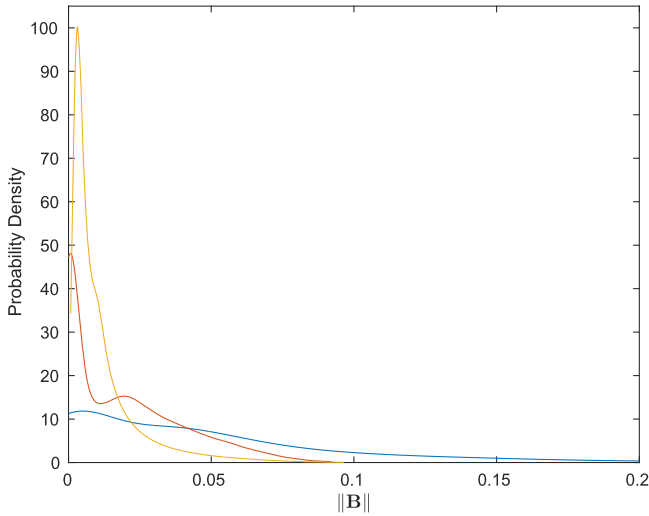
Figure 5. KDEs of \|B\| in an OCR. Key: potential (yellow), full MHD (blue), modified density (orange).
