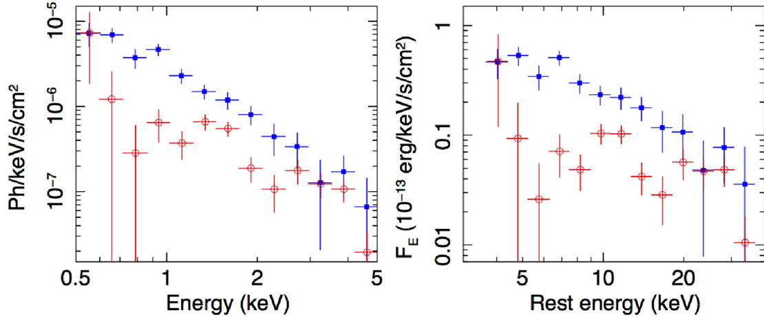
Fig. 5. Comparison between the 2003 XMM-Newton (in blue) and 2017 Chandra (in red) spectrum of SDSS J1030+0524. Both spectra have been corrected for the effective response. The XMM-Newton spectrum is the average of the three EPIC cameras (with S/N weighting). The left panel shows the observed-frame spectra, while the right panel shows the rest-frame one.
