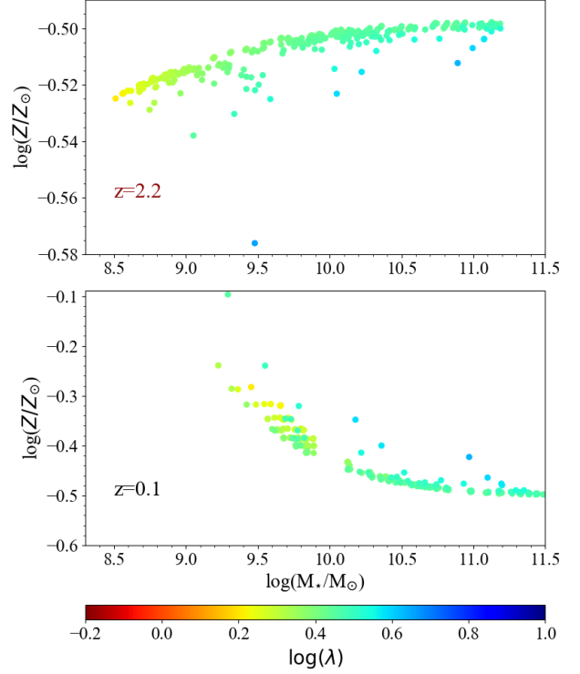
Fig. 20. Stellar mass-metallicity relation for the galaxies which follow the Mignoli et al. (2019) MZR and the high redshift star forming main sequence by Pearson et al. (2018) computed at redshift z = 2.2 (upper panel) and z = 0.1 (lower panel).
