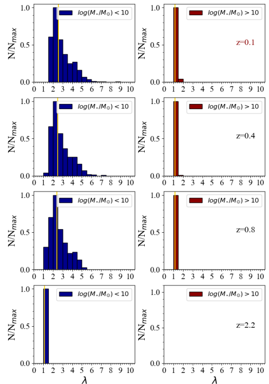
Fig. 14. As in Fig. 4, but computed with the local MZR proposed by Curti et al. (2020).
