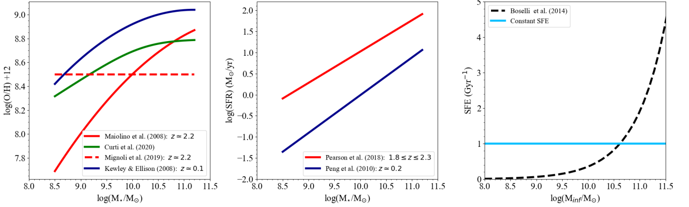
Fig. 1. Left panel: Observed MZR adopted in this paper at different redshifts: the local one by Kewley & Ellison (2008) is depicted with the blue line, the high redshift MZR by Maiolino et al. (2008) with the red one. The red dashed line is the MZR observed by Mignoli et al. (2019) at z \sim 2 . With the solid green line we also show the local MZR relation for SDSS galaxies found by Curti et al. (2020) with a fully T_e -based abundance scale analysis. Middle panel: The star-forming main sequence by Peng et al. (2010) in local SDSS galaxies is shown with the blue line, whereas the high redshift relation is the one by Pearson et al. (2018). Right panel: With the dashed black line we show the star formation efficiency as a function of the infall mass M_{\text{inf}} from the scaling relation for the gas depletion timescale as found by Boselli et al. (2014). The constant SFE fixed at the value of 1 \text{ Gyr}^{-1} is indicated with the light blue curve.
