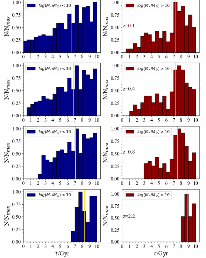
Fig. 5. As in Fig. 4, but in each panel the plotted distribution is for the infall time-scale parameter \tau .
