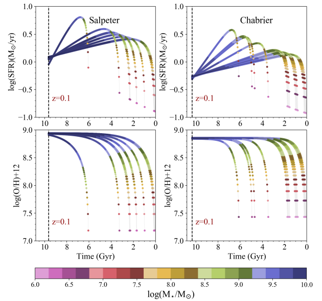
Fig. A.6. Evolution of star formation rate (upper panels) and oxygen abundance (lower panels) as a function of time for the galaxies with infall mass M_{\text{inf}} = 10^{10.5} M_{\odot} which lie on the MZR of Kewley & Ellison (2008) and on the MSR as derived by Peng et al. (2010) , computed assuming a Salpeter (1955) IMF (left panels) and a Chabrier (2003) IMF (right panels). The colour coding stands for the stellar mass.
