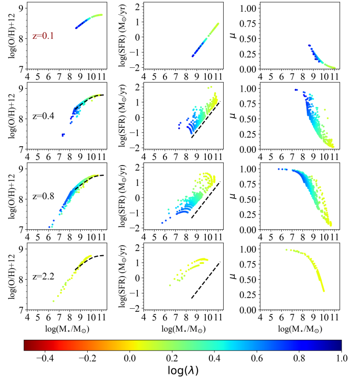
Fig. 13. Backward evolution from z = 0.1 to z = 2.2 of the galaxies which obey the analytical fit of the observed MZR at z \sim 0.1 of Curti et al. (2020) and the local main sequence of star-forming galaxies as derived by Peng et al. (2010), colour coded as a function of the loading factor parameter \lambda as in Fig. 2. The black dashed lines in the panels of the first column and in each \text{SFR}-\log(M_{\star}/M_{\odot}) plot, show the MZR of Curti et al. (2020) and the MSR derived in local star-forming galaxies by Peng et al. (2010), respectively.
