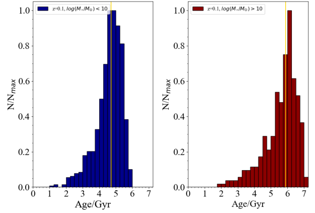
Fig. A.5. Age distribution for star-forming galaxies which are on the MZR at z = 0.1 in two different mass bins as in Fig. 7, computed assuming a Chabrier (2003) IMF.
