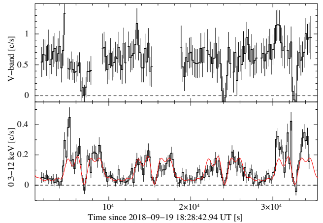
Figure 1. 2018 September 19 OM Vband (upper panel) and PN 0.3–12 keV (lower panel) background subtracted light curves binned at 200 s, where for plotting purposes is also shown the result of a fit made with seven sinusoids, the orbital period (8565 s), and its first six harmonics (red curve).
