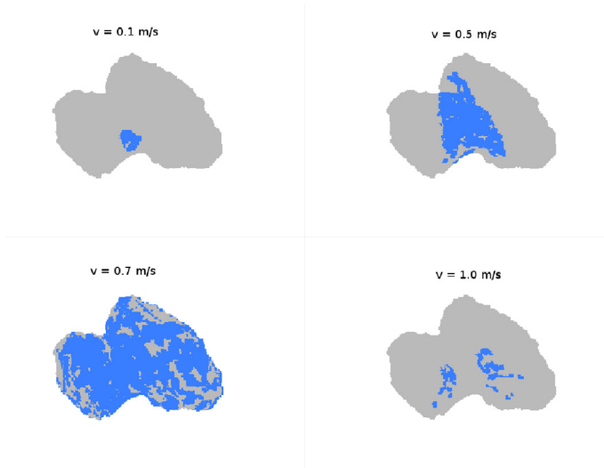
Fig. 10. As Fig. 9, but viewed from above the north pole, illustrating the extensive coverage of the northern hemisphere of the nucleus for ejection speeds of about 0.7 m/s.
