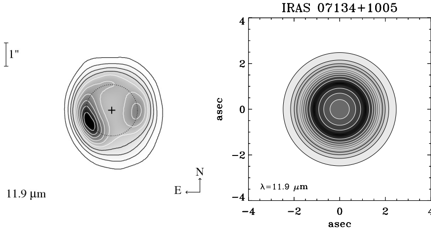
Fig. 2. Left: image of IRAS 07134+1005 observed at 11.9\ \mu\text{m} by Hony et al. (2003). Right: the map simulated at 11.9\ \mu\text{m} using the DUSTY code, assuming the parameters reported in Table 4. The map has been convolved with a circular beam with an HPBW of 0''.83 . In both the maps, the contours indicate the 5–95% intensity levels in steps of 10%.
