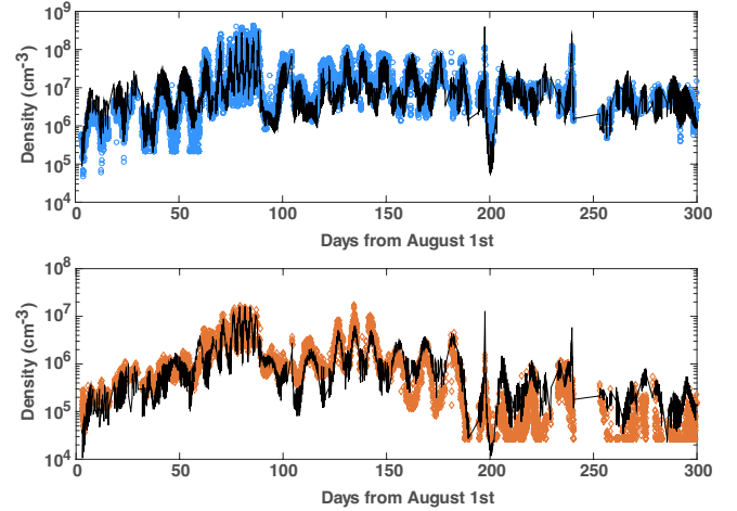
Fig. 3. Best fit of the analytical model (black) resulting from the optimization procedure with the DFMS data (blue for \text{H}_2\text{O} and orange for \text{CO}_2 ) from 4 August 2014 to 2 June 2015.
