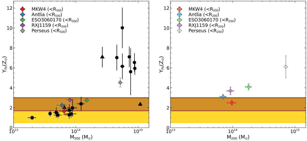
Figure 4. Left-hand panel: Effective Fe yield as a function of cluster/group mass within R_{500} . The circles represent Fe yield for the cluster in the sample of Ghizzardi et al. (2021), squares represent the groups in the sample of Renzini & Andreon (2014), triangles represent NGC 1550, Hydra A, and Coma in the sample of Sasaki, Matsushita & Sato (2014). The yellow shaded region shows the expected value estimated from the SN yields derived from Maoz & Graur (2017) and Renzini & Andreon (2014). The brown shaded region shows the expected value calculated assuming higher SNIa rate from Freundlich & Maoz (2021). Right-hand panel: Effective Fe yield as a function of cluster/group mass within R_{200} .
