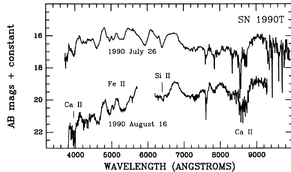
FIG. 4. Spectral evolution of SN 1990T. The spectra are plotted on an AB magnitude scale ( AB = -2.5 \log f_v + \text{constant} ), shifted with respect to each other by arbitrary amounts.
