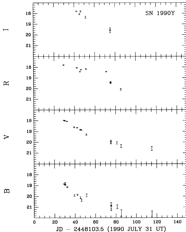
FIG. 7. B , V , R , and I light curves of SN 1990Y.
