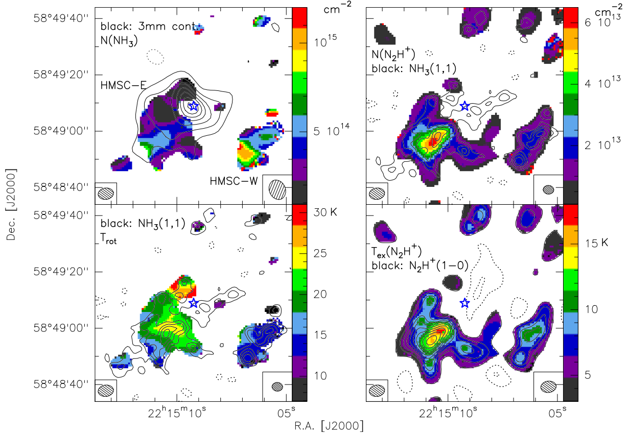
Fig. 9. Left: NH 3 column density map ( top ) and rotational temperature map overlaid with 3 mm continuum and NH 3 (1, 1) integrated intensity contours, respectively. Right: the N 2 H + column density map overlaid with NH 3 (1, 1) integrated intensity contours ( top ), and N 2 H + (1–0) excitation temperature map overlaid with N 2 H + (1–0) integrated intensity contours. The 3 mm continuum contours start at 3\sigma in steps of 4\sigma . All the other contour levels parameters are the same as in Fig. 5. The synthesized beam of the temperature and column density map is shown in the bottom left corner of each panel, and the synthesized beam of the contour map is shown in the bottom right corner of each panel.
