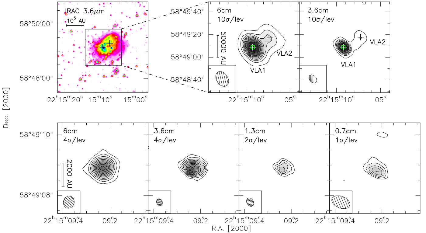
Fig. 1. Spitzer /IRAC and (E)VLA continuum emission images. Top: Spitzer /IRAC 3.6 \mu\text{m} , ELVA (D-config) 6.0 cm and 3.6 cm continuum images. Bottom: the VLA 6.0 cm (A-config), 3.6 cm (A-config), 1.3 cm (B-config), and 0.7 cm (C-config) continuum images. The boxes in the EVLA continuum images in the top indicate the zoomed region in bottom panels . All the contour levels start at 4\sigma , and the steps are shown in each panel. The \sigma values are listed in Table 4. The crosses in the top panels mark the two radio sources we detected. The synthesized beams are shown in the bottom left corner of each panel. The Spitzer /IRAC post-bcd data processed with pipeline version S18.25.0 have been downloaded from the Spitzer archive to create the image.
