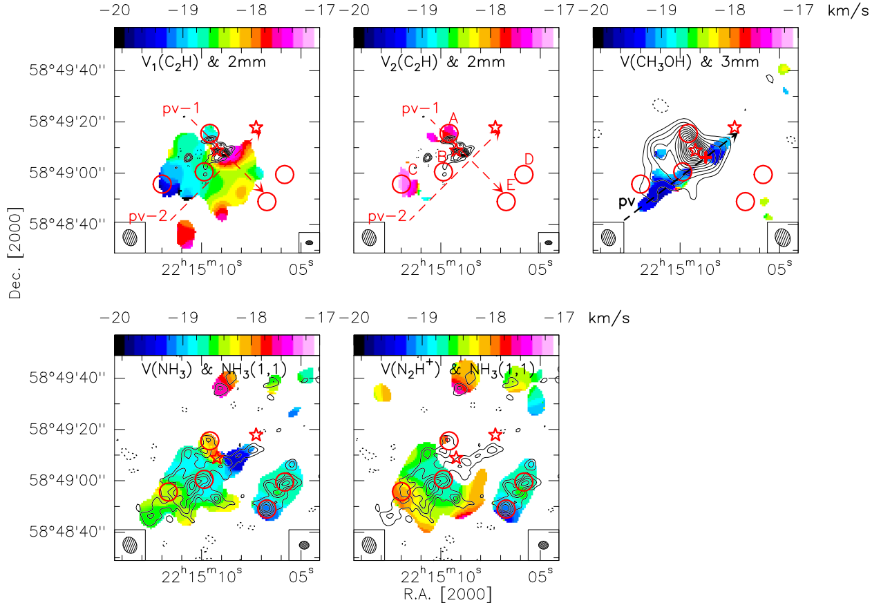
Fig. 10. Molecular line velocity maps overlaid with 2 mm, 3 mm continuum map and the \text{NH}_3(1, 1) integrated intensity map. The contour level parameters are the same as the ones in Figs. 3 and 5. The dashed arrows in the top panels mark the PV-cuts used for PV diagrams in Fig. 13. The star marks the UCHII region. The cross in the top right panel indicates the reference position in \text{CH}_3\text{OH} PV diagram in Fig. 13. The circles indicate the area where the average spectra are extracted and shown in Fig. 14. The synthesized beam of the velocity maps is shown in the bottom left corner of each panel, and the one of the contours is shown in the bottom right corner of respect panel.
