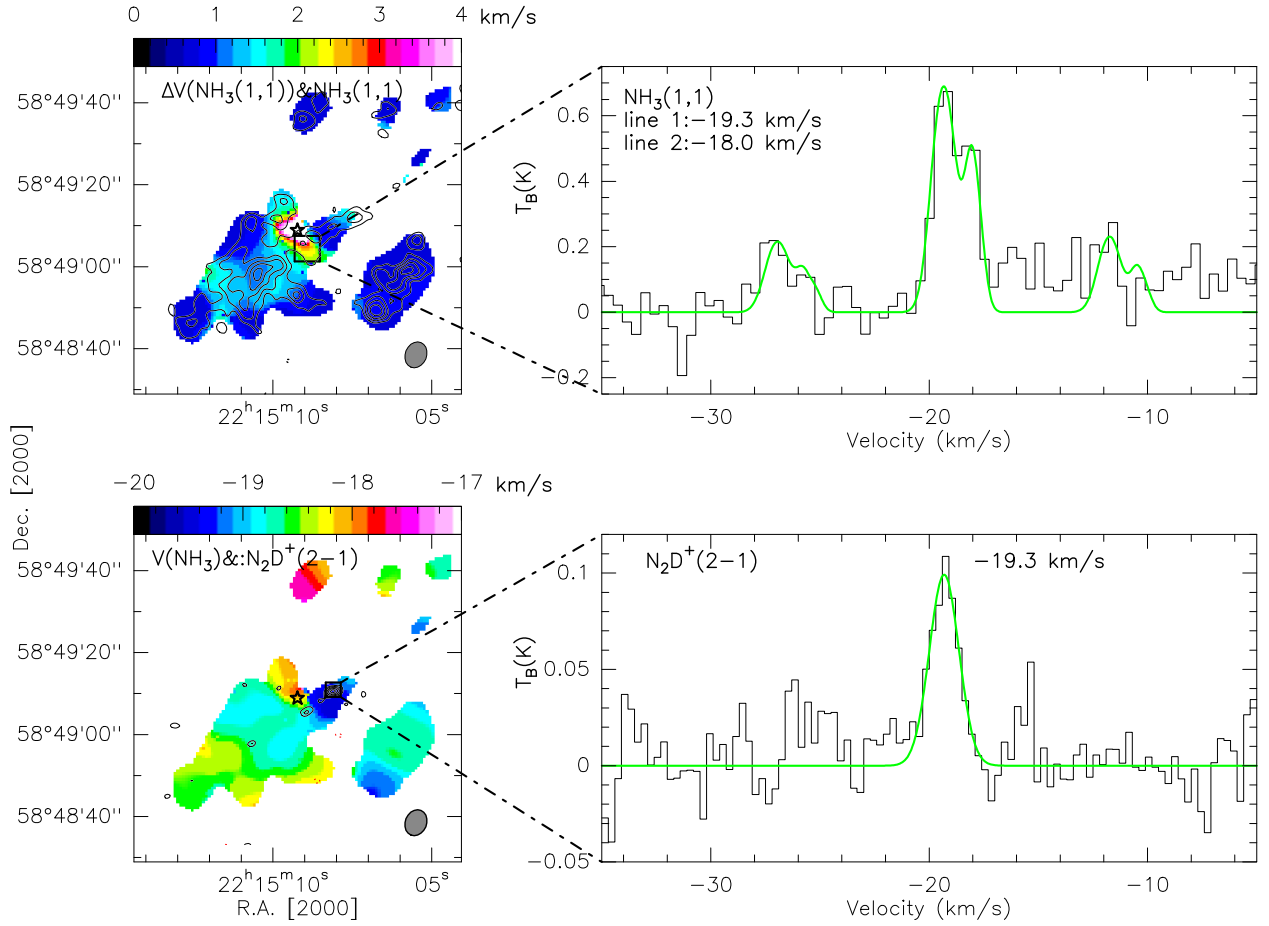
Fig. 12. Top: \text{NH}_3(1, 1) line-width map overlaid with the \text{NH}_3(1, 1) integrated intensity map and the average \text{NH}_3(1, 1) spectrum extracted from the region outlined with the box in the line-width map. Bottom: \text{NH}_3(1, 1) velocity map overlaid with \text{N}_2\text{D}^+(2-1) integrated intensity map, \text{N}_2\text{D}^+(2-1) average spectrum extracted toward the emission peak indicated with the box in the velocity map.
