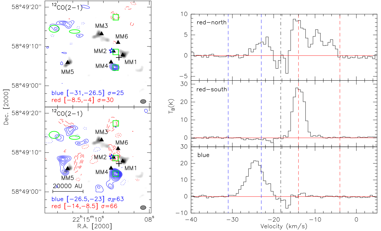
Fig. 6. SMA ^{12}\text{CO}(2-1) outflow maps overlaid with the SMA 1.3 mm continuum map (left), and the average ^{12}\text{CO}(2-1) spectra extracted from the peaks of the red- and blueshifted emission denoted by squares in the left panels. Top-left panel shows the high velocity outflow map, and the bottom left one shows the low-velocity outflow map. In both panels, the full and dashed contours show the blueshifted and redshifted ^{12}\text{CO}(2-1) outflow emission, respectively. All the contour levels start at 4\sigma and increase with a step of 2\sigma/\text{level} . The \sigma value and velocity-integration range of each outflow emission are shown in the bottom of the left panel in units of \text{mJy beam}^{-1} and \text{km s}^{-1} , respectively. Two open ellipses indicate the nebulous \text{H}_2 emission detected by Kumar et al. (2002). The cross marks the infrared source that was suggested by Palau et al. (2013) as the driving source of the outflow. The triangles indicate the positions of our 2 mm cores. The dotted contours are the negative features due to the missing flux with the same contour levels as the positive ones in the panel. The synthesized beam of the outflow map is shown in the bottom right corner of the left panel. The squares at the peaks of the red and blue outflow lobes with the size of 1''.4 \times 1''.4 show the area where we extracted the spectra shown in the right panels. In the right panels, the dashed lines indicate the velocity regimes we used to define the outflow emission, the dashed-dotted line marks the v_{\text{LSR}} = -18.3 \text{ km s}^{-1} .
