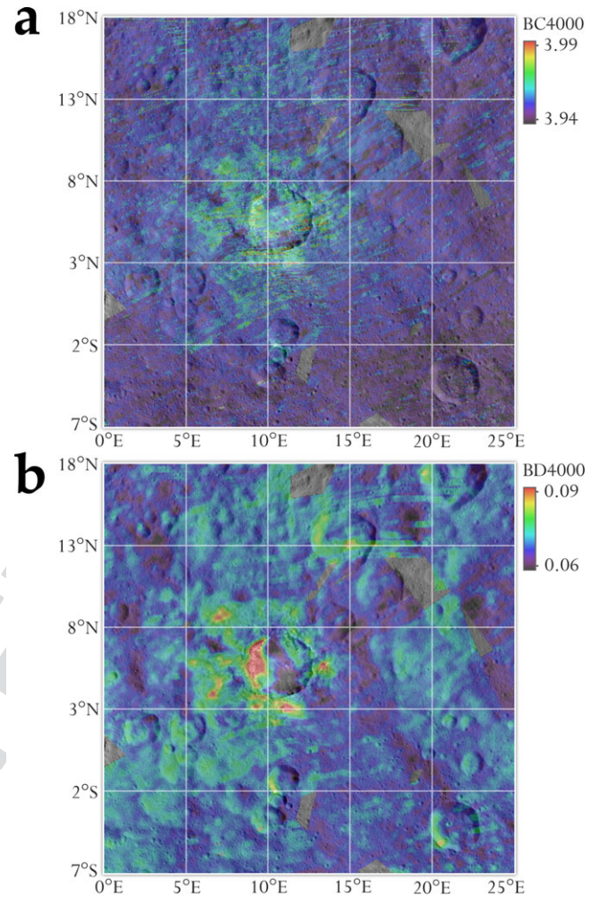
Fig. 7. Distribution of 4.0 \mu\text{m} 's band center (a) and band depth (b) values across the region of crater Haulani, derived from VIR data. These parameters are, respectively, sensitive to the composition and abundance of carbonate minerals. The overall distribution spans from Mg- or (Mg,Ca)-rich carbonates (violet to blue) to Na-rich carbonates (red) (a), and from lower depth (violet to blue) to greater depth (red) (b). The western and northwestern inner wall, the eastern inner wall and their respective rims, part of the floor, as well as part of the ejecta, appear enriched in Ca- and Na-rich carbonates compared to surrounding regions.
