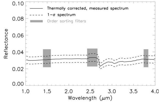
Fig. 1. Average spectrum of Ceres in the 25^\circ \times 25^\circ region roughly centered on crater Haulani, as measured by the VIR imaging spectrometer in the 1–4 \mu\text{m} spectral range during the HAMO mission phase at an average resolution of 0.38 km/px. The solid line represents the mean spectrum, while the dashed lines mark the 1- \sigma variability. All VIR spectra used to compute the average spectrum were first corrected for thermal emission, and then for illumination and observation geometry by means of a Hapke's model. Gray boxes highlight the spectral counterparts (position and width) of three-order sorting filters placed on top of the VIR infrared focal plane, which induce systematic artifacts in VIR spectra. The spectral signatures diagnostic of Mg-bearing phyllosilicates and \text{NH}_4 -bearing phyllosilicates are centered at 2.72–2.73 \mu\text{m} and 3.06 \mu\text{m} , respectively. The carbonates' signatures, at 3.3–3.5 \mu\text{m} and 3.95–4.01 \mu\text{m} , are much weaker compared to the previous features.
