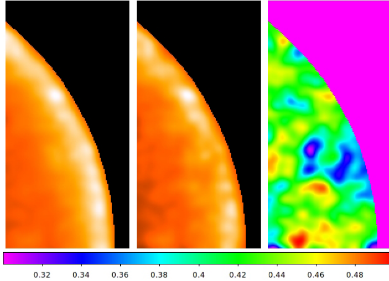
FIGURE 3. Simulated 4-6 keV maps of polarised synchrotron radiation of a supernova shell with turbulent magnetic field. 4-6 keV intensity is shown with a linear colour scale in the left-hand panel. The right-hand panel shows the degree of polarisation indicated by the colour bar. The stochastic magnetic field sample has Kolmogorov type spectral index = 5/3 . The central panel shows the product of intensity and polarisation degree (see [18]).
