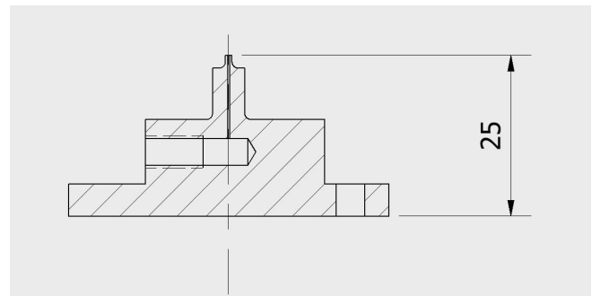
Figure 5. Picture and technical draw of the prism holder.
