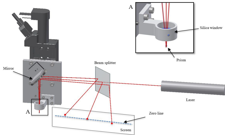
Figure 6. Overall picture of the clock control system.
