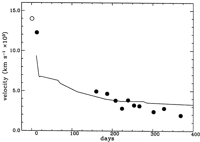
Fig. 7. Temporal behaviour of the width (FWHM) of H\alpha emission. The open symbol represents a measurement reported in IAU 4965. For comparison, the data of SN 1987A from the ESO data set are also reported
