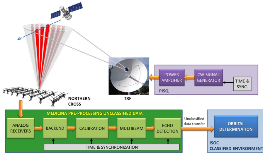
Figure 3: BIRALES system architecture.
