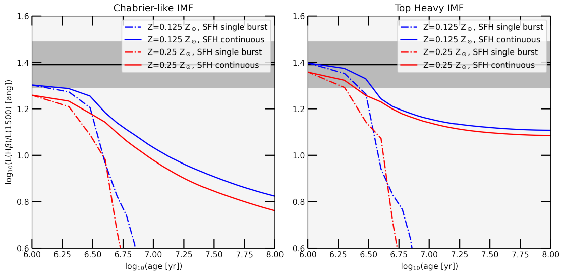
Figure 8. Theoretical tracks of the evolution of the L(\text{H}\beta)/L_V(1500\text{\AA}) (rest-frame) with stellar population age, and depending on the IMF: Chabrier-like (left panel) or top-heavy (right panel). The tracks are colour-coded according to the stellar metallicity adopted, 0.125 Z_\odot (blue tracks) and 0.25 Z_\odot (red tracks). Besides, they are reported with a solid line if the SFH used in the modelling is continuous, or with a dashed-dotted line in the case of a single burst model. The tracks have been obtained from the synthetic models of Starburst99 (Leitherer et al. 1999). The horizontal black solid line shows our estimate of the L(\text{H}\beta)/L_V(1500\text{\AA}) ratio while the grey-shaded area is indicative of its associated error.
