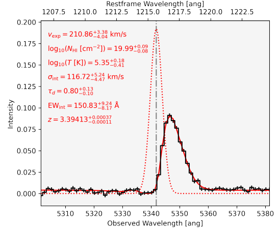
Figure 6. Diagram showing the \text{Ly}\alpha intensity spectrum (black solid line) and the best-fit model (red solid line) obtained by means of the radiative transfer code tlac (Gronke & Dijkstra 2014). The red dotted line shows the reconstructed shape of the intrinsic \text{Ly}\alpha emission, while the vertical dashed-dotted line shows the expected position of the \text{Ly}\alpha line according to the systemic redshift.
