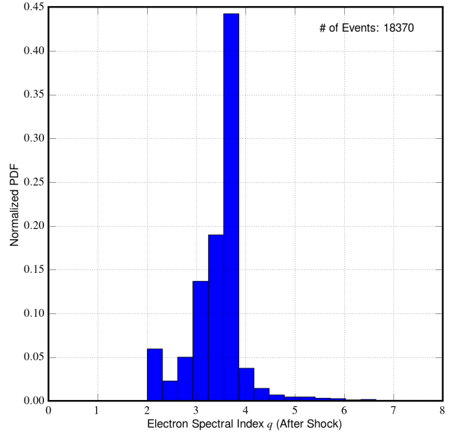
Figure 12. Normalized PDF of the modified spectral slope q as the particle crosses the shock during the evolution of slab jet until 0.3 Myr.
