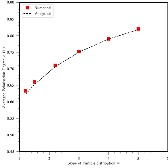
Figure 8. Comparison of the numerically estimated averaged ratio of J_{sy}(\nu) with J_{pol}(\nu) for \nu = 10^{10} \text{GHz} (red squares) with the theoretical values obtained from Eq. 71 shown as black dashed line.
