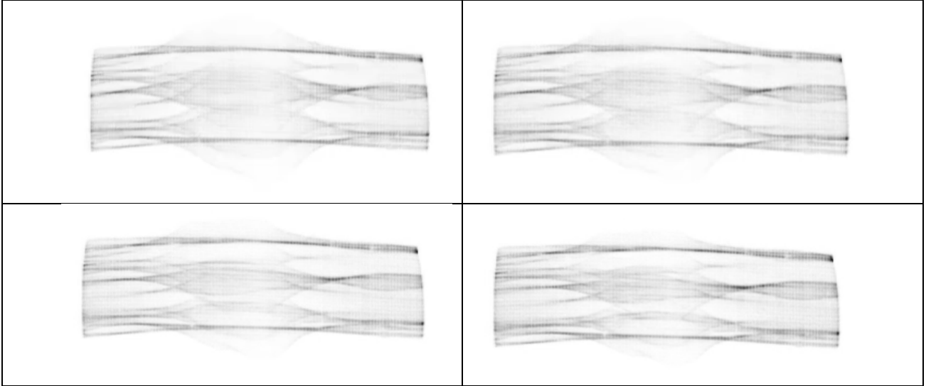
Fig. 16: second sector of the XSM, illuminated at 0.3 keV: voltage ramp of the 7 piezos together at 0 V (top left), -60 V (top right), -80 V (bottom left), -90 V (bottom right), at an incidence angle of 2.7 deg. We note the deformations induced by the glue on the glass foil, visible as broadening of the striations, progressively corrected for increasing negative voltages.
