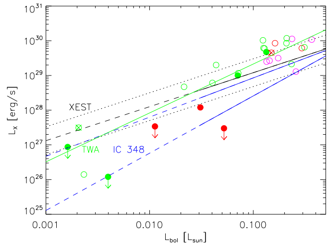
Figure 2. X-ray vs. bolometric luminosities for TWA M-type stars, with symbols as in Figure 1. The best-fit linear regression is indicated as a green line. The empirical relationships between L_X and L_{bol} inferred for low-mass T Tauri stars and young brown dwarf candidates in Taurus (Grosso et al. 2007) and for low-luminosity stars in IC 348 (Stelzer et al. 2012) are indicated by the black and (two) blue lines, respectively; the two lines for IC 348 are the results of linear regression results for Class II and Class III pre-MS stars (lower and upper blue lines, respectively). The dashed portions of the black and blue lines indicate extrapolations of the linear regressions of L_X vs. L_{bol} for Taurus and IC 348, and the dotted black lines indicate the approximate 1\sigma scatter for the Taurus sample.
