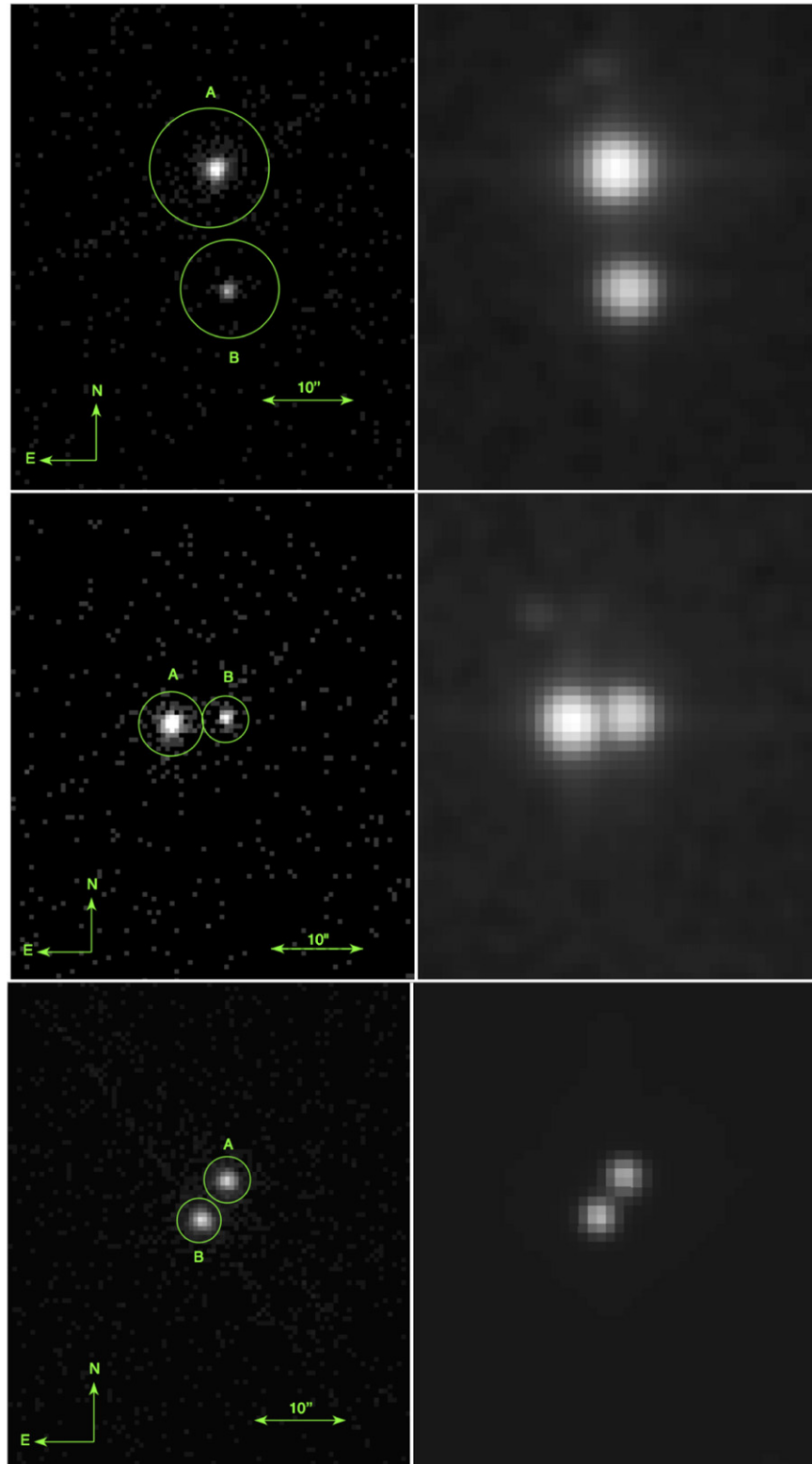
Figure 3. Chandra /ACIS-S3 images of TWA 8 (top), 9 (middle), and 13 (bottom), with orientation and scale indicated, alongside 2MASS J band images of the same systems at the same orientation and scale.
