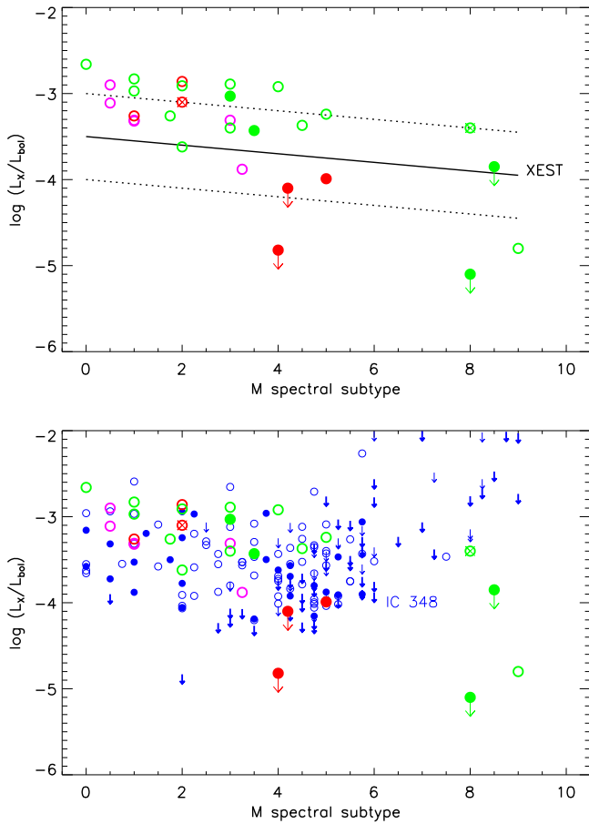
Figure 1. Top: \log of the ratio of X-ray to bolometric luminosity for TWA M-type stars, plotted as a function of spectral subclass. Magenta, red, and green symbols indicate ROSAT , XMM , and Chandra observations, respectively. Filled and open circles represent stars with and without warm circumstellar dust, i.e., with and without detectable mid-IR excesses; an “X” indicates the IR excess status of the star is unknown (see Table 1). The solid line indicates the dependence of \log(L_X/L_{bol}) on spectral type, and dashed lines indicate the 1\sigma scatter in \log(L_X/L_{bol}) , as determined by Grosso et al. (2007) for low-mass T Tauri stars and young brown dwarf candidates that were included in the XMM-Newton extended survey of Taurus (XEST; Güdel et al. 2007). Bottom: as in the top panel, with blue symbols indicating measurements of \log(L_X/L_{bol}) for low-luminosity stars in IC 348 (Stelzer et al. 2012), where filled and open circles represent X-ray-detected pre-MS stars with disks (Class II) and without disks (Class III), respectively (and thick and thin arrows indicate X-ray-nondetected stars of these respective classes).
