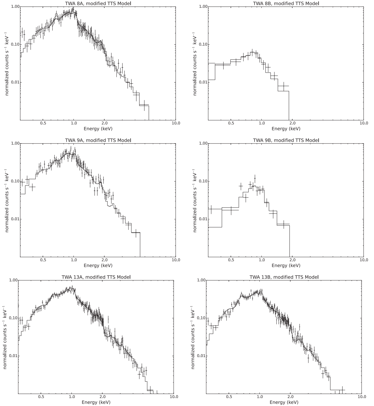
Figure 4. Chandra /ACIS X-ray spectra (crosses) of the A (left) and B (right) binary components of the TWA 8 (top row), 9 (middle row), and 13 (bottom row) systems, with best-fit two-component absorbed plasma models (histograms) overlaid.
