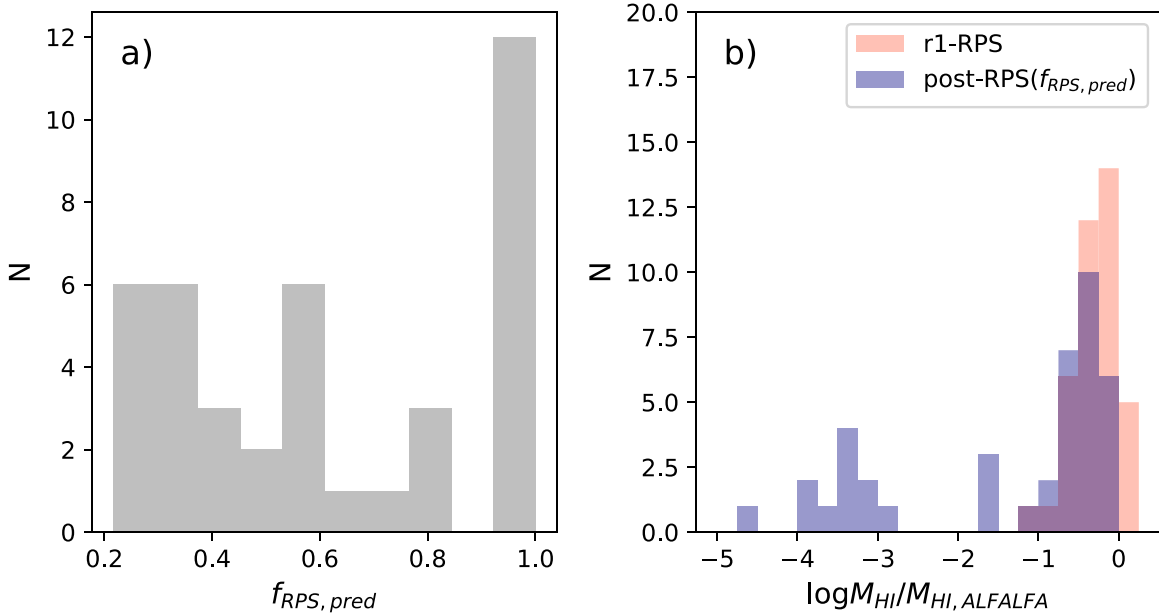
Figure 6. Distributions of the RPS strengths for the r1-RPS candidates. Panel (a) plots the predicted mass fraction of strippable H I ( f_{\text{RPS,pred}} ). Panel (b) plots the difference of M_{\text{HI}} at a given M_* with respect to the ALFALFA mean relation of M_{\text{HI}} vs. M_* ( \log M_{\text{HI}}/M_{\text{HI,ALFALFA}} ). The distributions of \log M_{\text{HI}}/M_{\text{HI,ALFALFA}} at the present and in the post-RPS status after removing the strippable H I (i.e., M_{\text{HI}}(1 - f_{\text{RPS,pred}})/M_{\text{HI,ALFALFA}} ) are plotted in red and blue, respectively.
