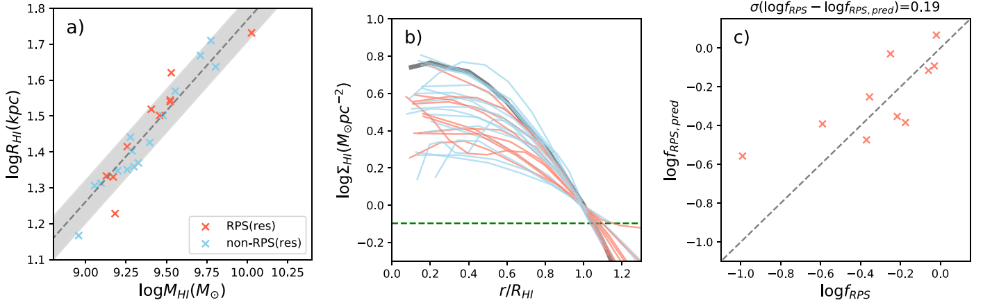
Figure 2. Radial measurements of H I for the 27 well-resolved galaxies. Panel (a): the size–mass relation of H I. The sizes R_{\text{HI}} have been corrected for the effect of beam smearing as R_{\text{HI}} = \sqrt{R_{\text{HI,obs}}^2 - b_{\text{maj}}^2} , where R_{\text{HI,obs}} is directly derived from the H I images as the semimajor axis of the ellipse with a de-projected surface density of 1 M_{\odot} \text{pc}^{-2} . The mean relation and scatter from Wang et al. (2016) is plotted as the gray line and shaded region. Panel (b): the radial profiles of the H I surface density \Sigma_{\text{HI}} . The projection correction has been applied assuming an infinitely thin disk and an axis ratio determined from the optical light. The radii are normalized by R_{\text{HI}} . The median profile of 168 late-type galaxies (Wang et al. 2016, 2020a) is plotted as a gray, thick curve. The green dashed line marks \Sigma_{\text{HI}} = 0.8 M_{\odot} \text{pc}^{-2} corresponding to the detection limit of the WALLABY data. Panel (c): predicted vs. observed fraction of strippable H I mass over the total H I mass ( f_{\text{RPS}} ) for the resolved-RPS candidates. The predicted fraction f_{\text{RPS,pred}} has been corrected by multiplying by a factor of 1.4 (see text), in order to match the observed f_{\text{RPS}} on the one-to-one line. The 1\sigma rms of the difference between the two quantities are 0.19 dex, which drops to 0.14 dex if we exclude the one outlier which has f_{\text{RPS}} close to the threshold of 0.1 for identifying RPS candidates. In all panels, RPS (non-RPS) candidates are in red (blue).
