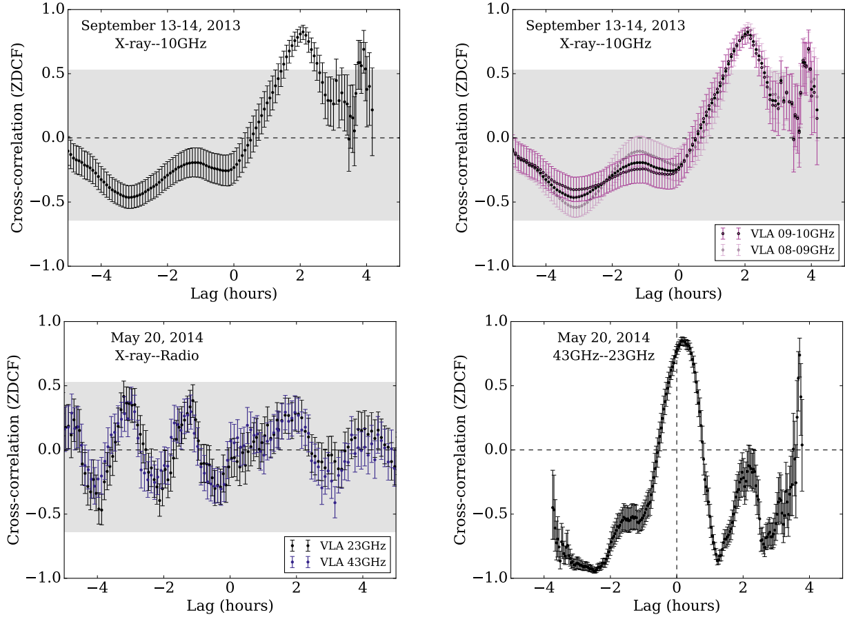
Figure 5. The ZDCF for the X-ray and radio light curves for 2013 September 14 (top panels) and for 2014 May 20 (bottom panels). The left panels are the cross-correlation between the X-ray and the average of all the radio spectral windows. The top right panel shows the cross-correlations between the X-ray and different radio frequency groupings. The bottom right panel shows the cross-correlation between two different JVLA frequency bands for 2014 May 20. A positive lag indicates structure appearing in the second data set (radio) after structure appears in the first (X-ray). The gray shaded regions denote the 2\sigma error interval from the null hypothesis testing (see §6.1).
