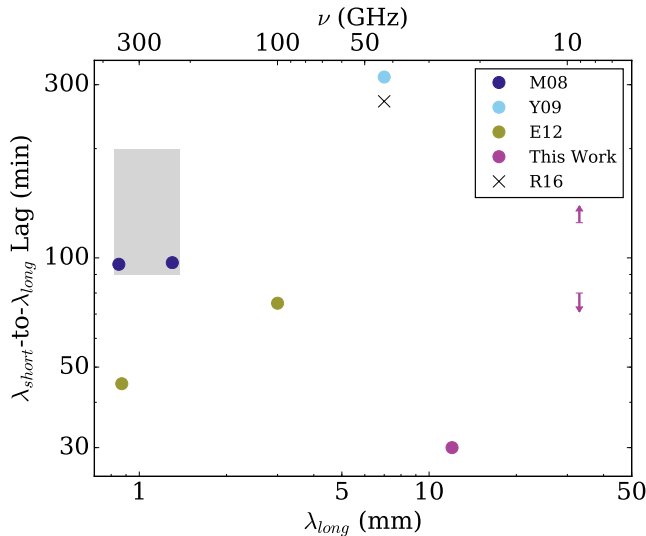
Figure 7. The X-ray or NIR ( \lambda_{short} ) to sub-mm or radio ( \lambda_{long} ) time lags for reported flares in the literature and three flares reported in this work. The colored points correspond to X-ray flares, while the gray box and gray ‘x’ correspond to NIR-only flares. The references in the legend are Marrone et al. (2008, M08) , Yusef-Zadeh et al. (2009, Y09) , Eckart et al. (2012, E12) , and Rauch et al. (2016, R16) .
