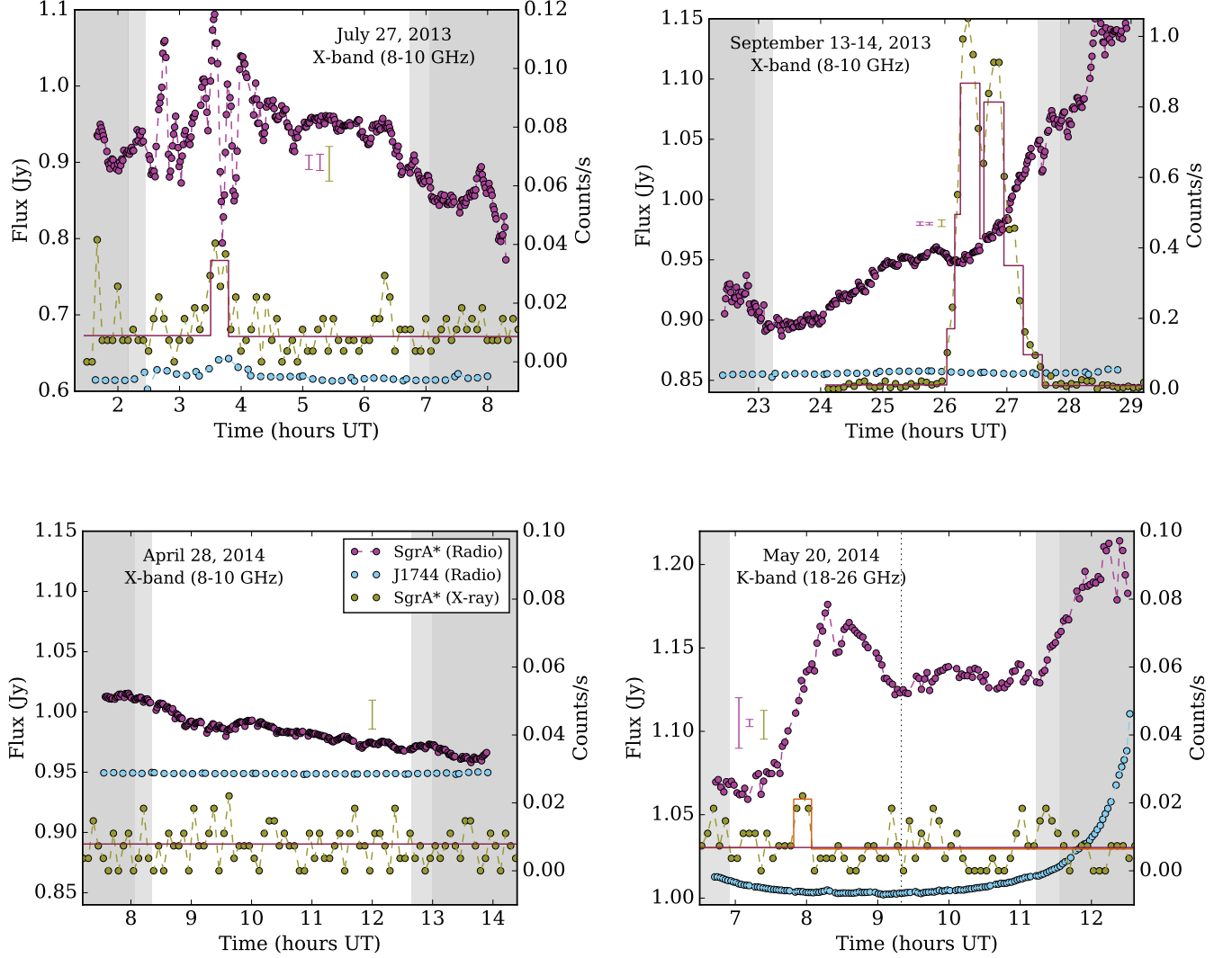
Figure 1. The Sgr A* and phase calibrator radio (purple and blue, respectively) and X-ray (green) light curves for three observations with significant radio variability (2013 July 27, 2013 September 14, and 2014 May 20). The bottom left panel (2014 April 28) shows a non-flaring radio observation. The darker gray shaded regions denote the time intervals where both SgrA* and the phase calibrator, J1744–3116, were below 18 degrees on the sky, and the lightly shaded regions mark times where only J1744–3116 is below 18 degrees. The phase calibrator is shifted by a constant factor for display purposes. The Bayesian Blocks results are overplotted in red for the X-ray light curves; the 2014 May 20 light curve includes an additional orange curve denoting the lower-confidence Bayesian Blocks results. Representative 2\sigma error bars are shown for the radio and X-ray light curves (for the radio, one error bar is for the entire observation and the other for just the higher elevation data in the non-shaded portion of the light curve; the error bar for the radio light curve for 2014 April 28 is too small to be visible on the figure).
