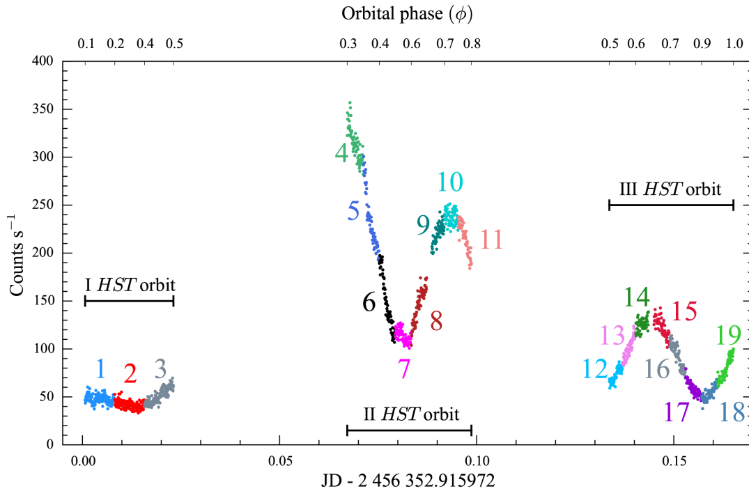
Figure 9. HST /COS light curve of SDSS1238, obtained over three consecutive spacecraft orbits, the gaps result from the target being occulted by the Earth. During the observations, the system showed an increase in brightness of \simeq 2 mag superimposed by a smaller amplitude ( \simeq 1 mag) sinusoidal variation on time-scales of half the orbital period. The colours highlight the different exposures from which the 19 subspectra have been extracted.
