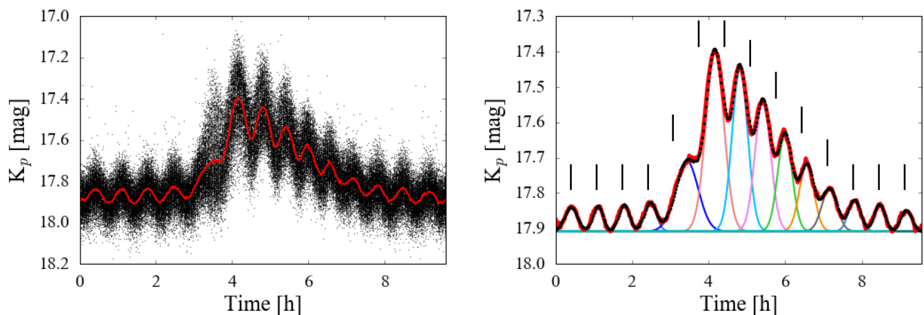
Figure 6. The 162 brightenings superimposed with respect to the 40.26 min ephemeris of the double-humps (left, black dots). The double-humped structure is clearly coherent throughout the K2 campaign, and shows an increase in amplitude during the brightenings. The red line represents the data binned over an interval of 5 s. The binned light curve is shown again on the right (red line, note the different scale of the y-axis) along with the best fit model (black, dotted), which is composed of a series of 14 Gaussians of different widths and amplitudes. The black ticks repeat regularly every 40.26024 min to show that the occurrence of the humps is delayed (i.e. they undergo a phase shift) during the brightening.
