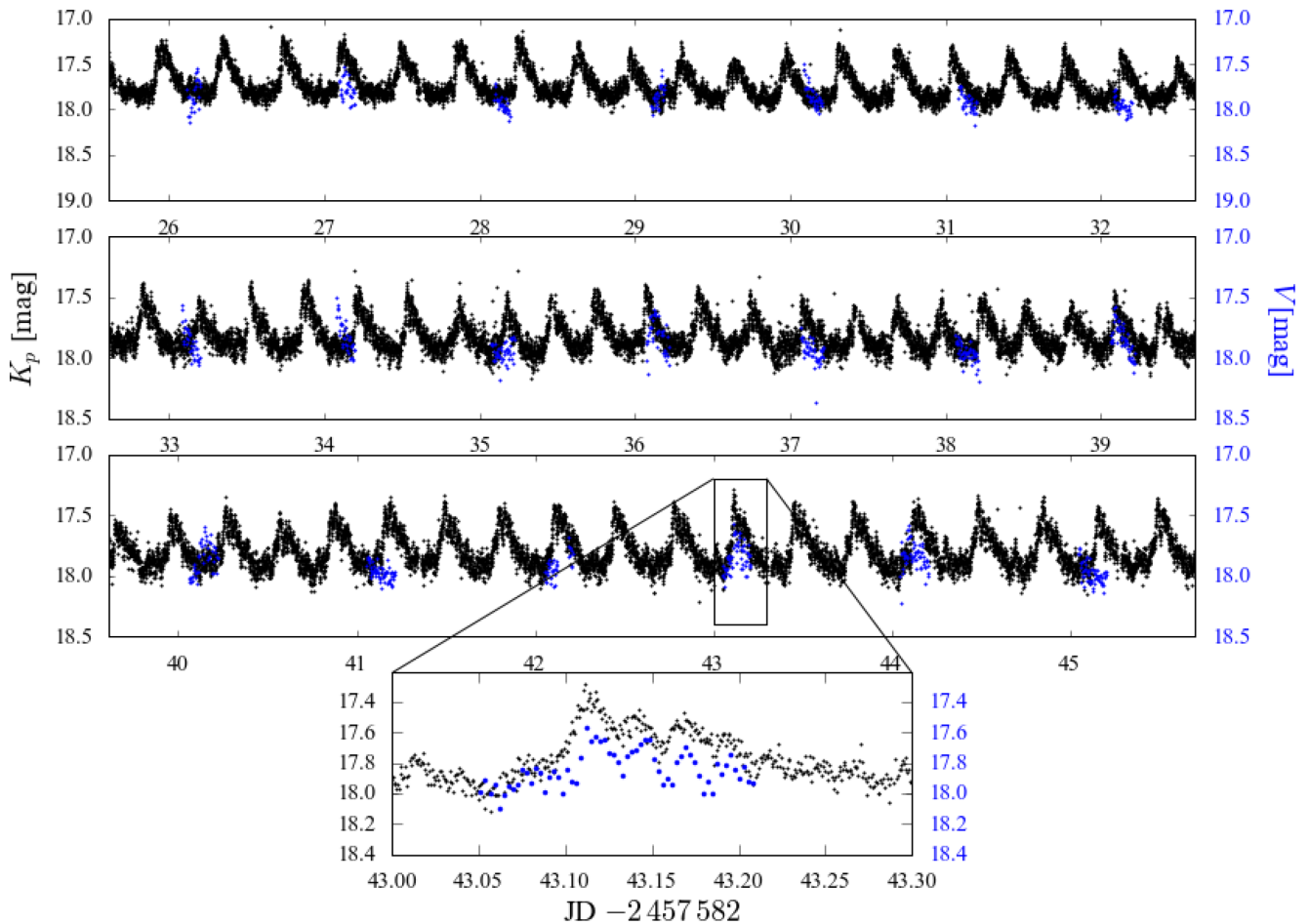
Figure 2. K2 light curve (black) from 2016 in comparison with V-band AAVSO observations (blue) acquired in a period of particular intense monitoring (20 February 2014 to 13 March 2014). The AAVSO data are shifted in time by \simeq 898.92 d to overlap with the K2 observations for an easy comparison. The quasi-period brightenings and the double-humps are clearly visible in both the data sets, showing the stability of both phenomena on time-scales of years.
