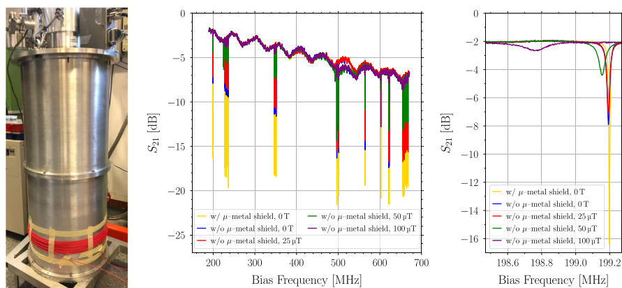
Fig. 6 Left panel: Picture of the testbed cryostat with a coil generating a tunable static magnetic field on the focal plane. Central panel: Amplitude of the S_{21} parameter measured, for the 31-pixel prototype, in dark conditions and at an operating temperature of 150 mK, under different magnetic fields. Right panel: Zoom on the first resonance of the central panel
