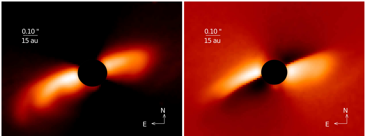
Fig. 2. IRDIS DPI Q_\phi ( left ) and U_\phi ( right ) images showing the close environment of RY Lup. The dark central region corresponds to the area masked by the coronagraph. The intensity scale follows the inverse hyperbolic sine.
