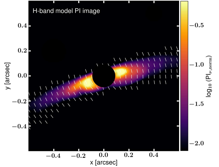
Fig. 10. Convolved polarized intensity H -band image considering a planet-induced spiral model with M_{\text{pl}}/M_\star = 1.4 \times 10^{-3} . The image is produced at an inclination of 75 deg, and a PAs of 107 deg. The inner 0.18'' are masked (black circular area) to mimic the coronagraph region. The white stripes represent the angle of linear polarization (fixed length, not scaled with the degree of polarization).
