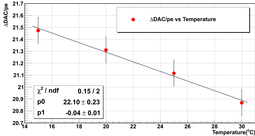
Figure 9. The variation of 50% trigger efficiency threshold versus temperature. The p0 and p1 are the intercept and the slope of the line of the best fit.
