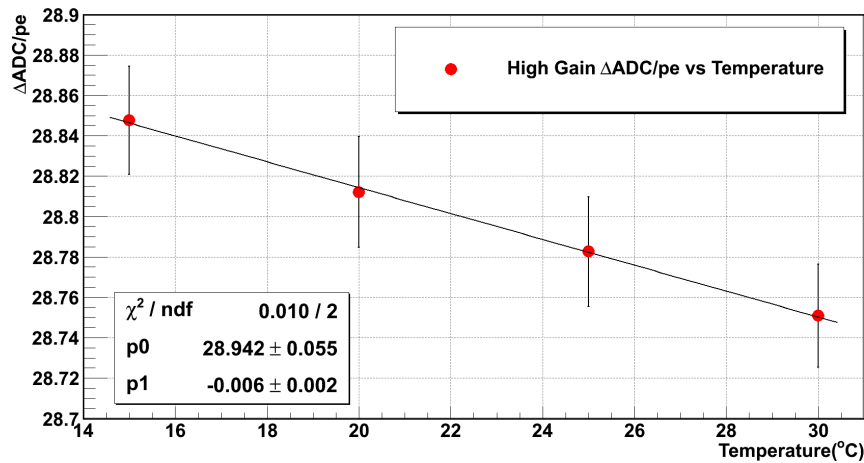
Figure 6. \Delta\text{ADC}/\text{pe} values versus temperature for the HG chain. The p_0 and p_1 are the intercept and the slope of the line of the best fit.
