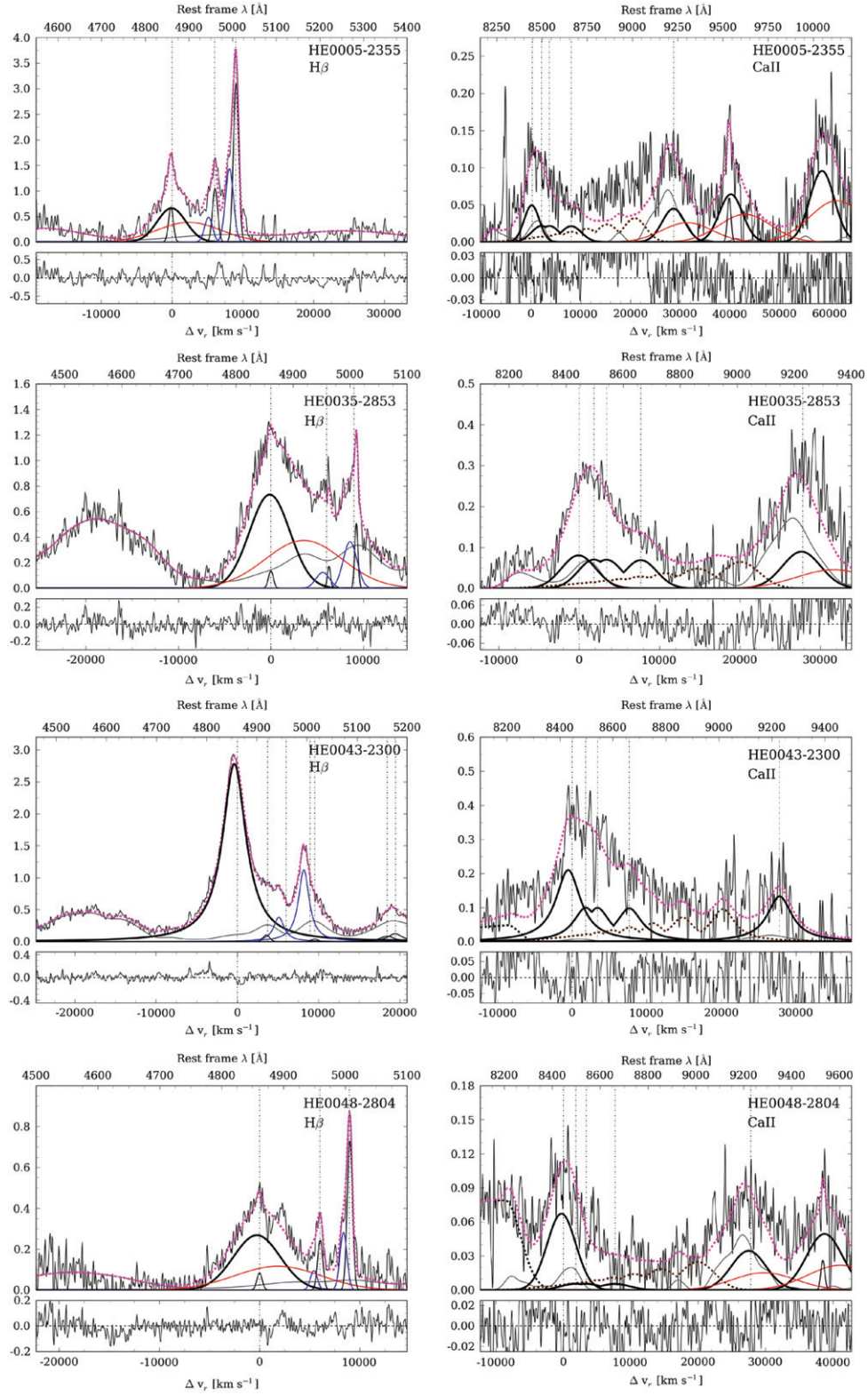
Figure 3. Quasar spectra after continuum subtraction. Abscissae are rest-frame wavelength in Å and ordinates are rest-frame specific flux in units of 10^{-15} \text{ erg s}^{-1} \text{ cm}^{-2} \text{ Å}^{-1} . The left panels show the H \beta spectral region and the right panels show the Ca II triplet spectral region. The vertical dashed lines are the rest frame H \beta , [O III] \lambda\lambda 4959, 5007 , O I \lambda 8446 and Ca II \lambda\lambda 8498, \lambda 8542, \lambda 8662 . Line coding is as follows. Thick black lines: broad components; thin black lines: narrow components; blue lines: blueshifted components of H \beta ; red lines: H \beta and Pa \gamma VBC; gray lines: Fe II contribution; thick dashed black lines: Paschen continuum; thick-brown lines: high-order Paschen lines; thin-dashed pink lines: best-fit model. Note that the Ca II triplet and high-order Paschen lines are shown as blends of individual lines and not as their sum.
