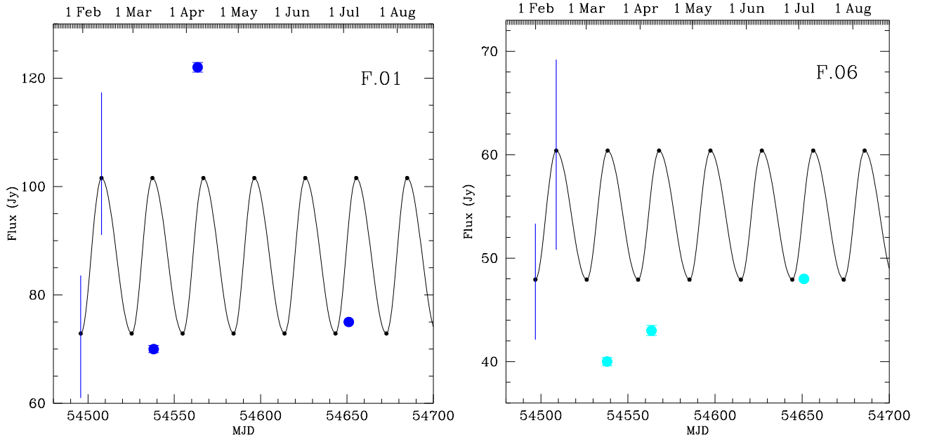
Fig. 5. Flux density versus time for the features F.01 ( left ) and F.06 ( right ). The black curve illustrates the expected variability of the maser feature according to Goedhart et al. (2009); the predicted times of maxima and minima are reported in Table 6. The blue bars indicate the range of the intensities between the highest maximum and the lowest maximum and between the highest minimum and lowest minimum.
