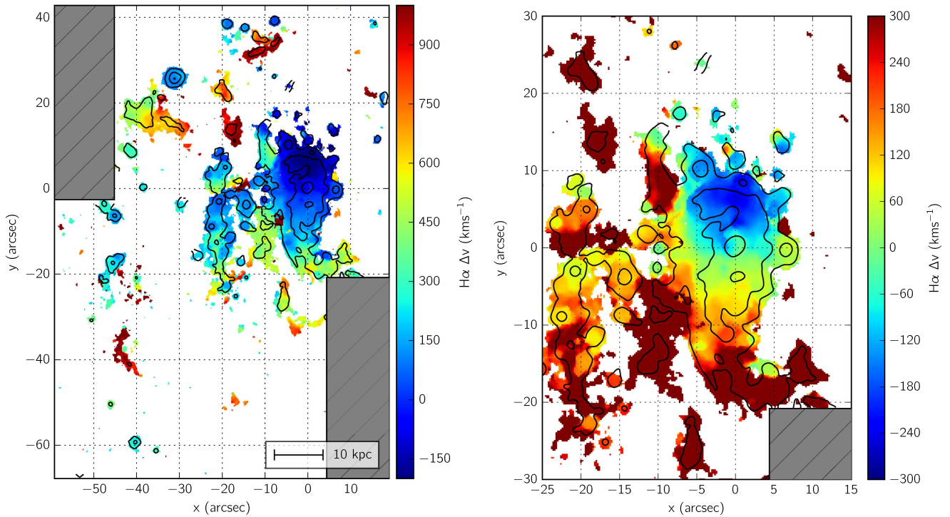
Figure 11. Left: velocity map of H \alpha ( \lambda 6562.82 ) emission relative to the galaxy systemic velocity comprised of a combination of single-component and two-component fits, as described in Section 4.2. The velocity map has been convolved with a median filter with a 3 \times 3 pixel kernel for visualization purposes, in addition to the data being smoothed using a mean filter with a 3 \times 3 kernel before fitting. Right: velocity map as on left, cropped to show the disk region with a rescaled color map to better exhibit the H \alpha kinematics of the disk region. Black contours in both panels indicate the H \alpha flux for context.
