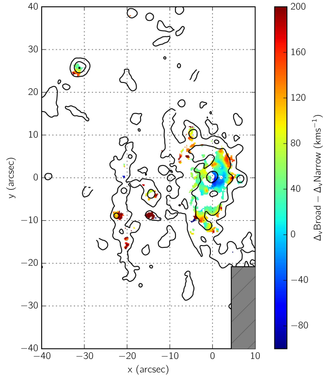
Figure 12. Velocity offset between the broad and narrow components of the H \alpha ( \lambda 6562.82 ) line where a double-component fit is available. The region of the blueward broad component, indicating a tail oriented toward the observer, is likely to originate from an outflow associated with the central AGN. The redward broad component in the outskirts of the disk evidences tails in the velocity distribution produced by increased stripping intensity at the outer edges of the disk. Black contours indicate the H \alpha flux for context.
