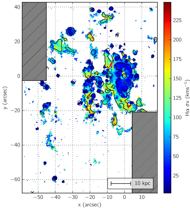
Figure 13. Velocity dispersion map produced using H \alpha ( \lambda 6562.82 ) emission from combined single-component and two-component fits as described in Section 4.2, corrected for instrument resolution by KUBEVIZ. The velocity dispersion map has been convolved with a median filter with a 3 \times 3 pixel kernel for visualization purposes.
