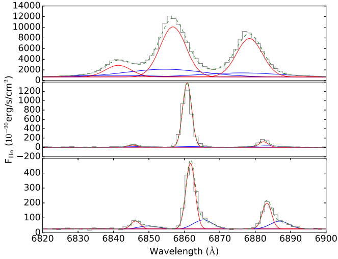
Figure 5. Observed H\alpha , N II emission-line group in three different spaxels within JO201 (black histograms), together with a two-component fit (the red and blue curves correspond to individual components, and the green dashed line is their sum). Top panel: central region of the galaxy, broadened by the AGN. Middle panel: region within the northeastern star-forming blob. Bottom panel: region in the outer part of the disk displaying obvious tails redward of the emission.
