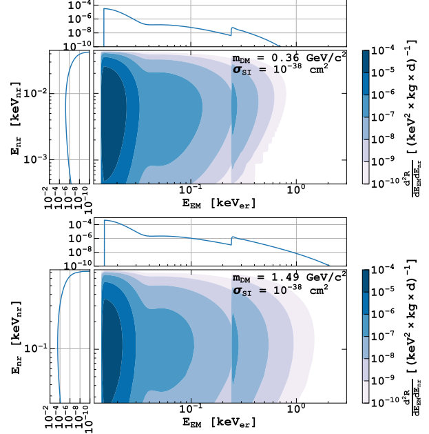
FIG. 1. 2D differential ionization rate as a function of the nuclear recoil energy ( E_{nr} ) and electromagnetic channel energy ( E_{EM} ) is shown for two representative DM masses, 0.36 GeV/c 2 (top) and 1.49 GeV/c 2 (bottom). The rate is given in events/(keV 2 kg d) and covers E_{EM} from 0.01 to 3 keV and E_{nr} from 4 \cdot 10^{-4} to 4 \cdot 10^{-2} keV for a DM mass of 0.36 GeV/c 2 and E_{nr} from 2.5 \cdot 10^{-2} to 7.5 \cdot 10^{-1} keV for a particle of mass 1.49 GeV/c 2 . The top and side panels of each figure depict the corresponding integrated distributions in the ME electron (top panels) and the NR (left panels) channels.
