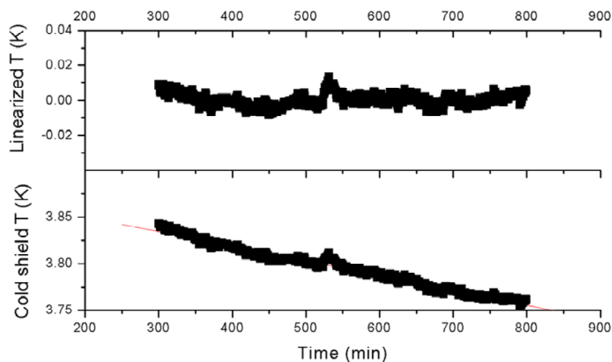
Figure 12: Fluctuation measured at the top of the cold shield. A linear drift is subtracted from the data to evaluate temperature fluctuations (upper panel)
