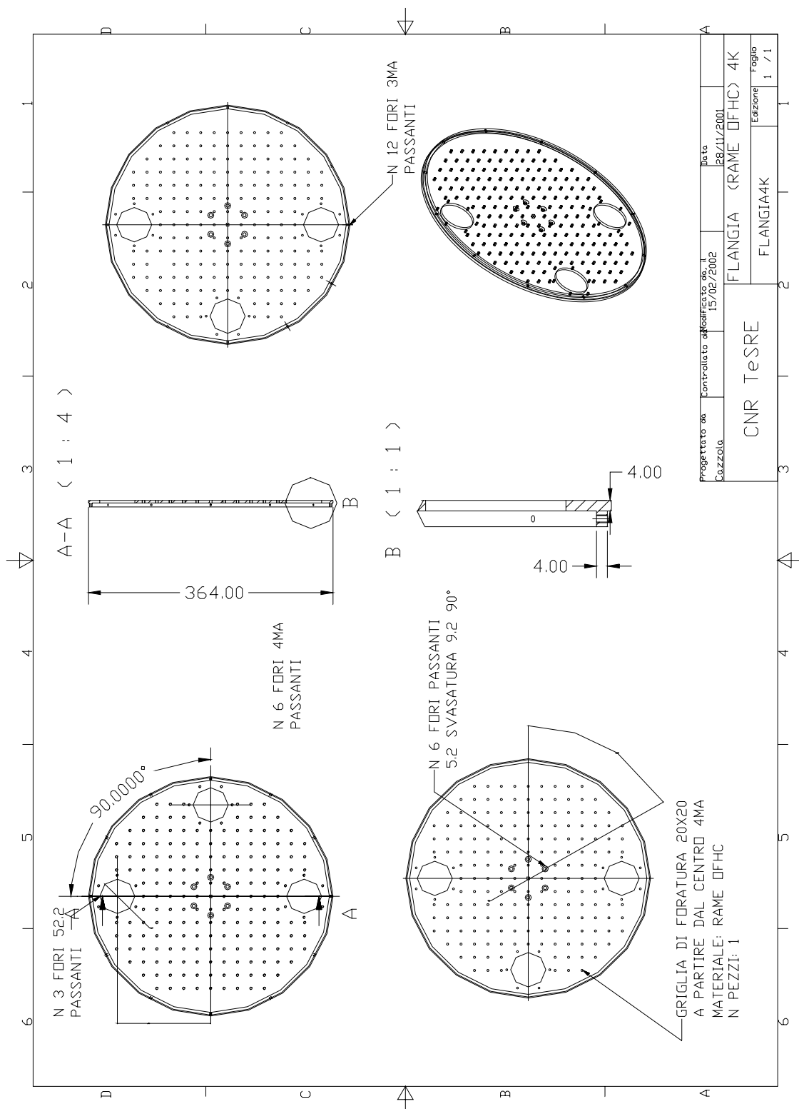
Figure 7: Drawing of the 4K flange made of OFHC copper
