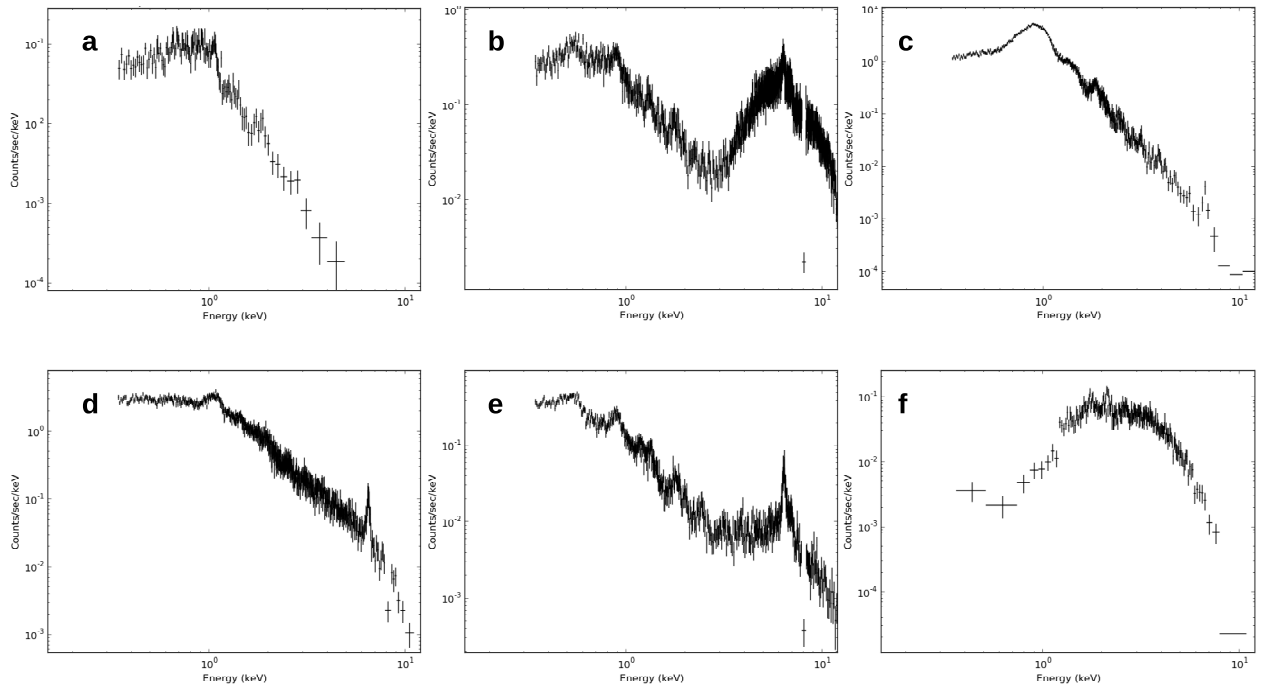
Fig. 13. Example spectra taken directly from the 3XMM catalogue, showing the diversity of the sources in the 3XMM catalogue. Energy (keV) is given on the abscissa and count \text{s}^{-1} \text{keV}^{-1} on the ordinate. a) 3XMM J052532.5+062533, an X-ray source of unknown nature, as the majority of the sources are in 3XMM b) 3XMM J123536.6-395433 a Seyfert 2 galaxy (NGC 4507) c) 3XMM J125141.9+273226, a rotationally variable star, 31 Com d) 3XMM J162838.2+393303, a cluster of galaxies e) 3XMM J011127.5-380500, the pn spectrum of NGC 424, a Seyfert 2 galaxy f) 3XMM J185246.6+003317, a new transient magnetar discovered by Zhou et al. (2014). Some low data points can be seen in the plots originating from pn data, but these are corrected for when the spectra are plotted in conjunction with the distributed response files.
