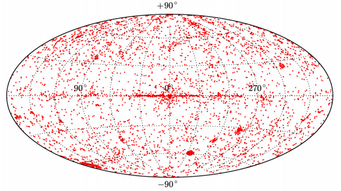
Fig. 1. Hammer-Aitoff equal area projection in Galactic coordinates of the 7781 3XMM-DR5 fields.
