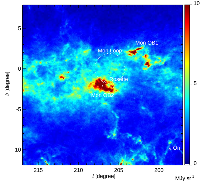
Fig. 1. The Rosette Nebula, its molecular cloud Mon OB2, and their surrounding medium as seen by Planck at 353 GHz. The dotted lines give the approximate outer radii of the Rosette H II region and the Mon Loop supernova remnant (described in Sect. 2). The northern Monoceros cloud Mon OB1 is above the Galactic plane; part of the dust ring of \lambda Ori is visible at the bottom right corner of the map; the northern end of Orion B is seen at (l, b) = (204^\circ, -12^\circ) (Dame et al. 2001).
