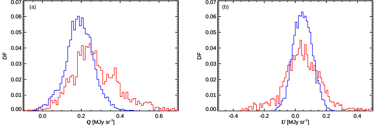
Fig. 4. Normalized distribution functions (DFs) of the (a) Stokes Q and (b) U maps measured within the background aperture (blue) and within the outer radius of the dust shell (red). The two regions are defined in Fig. 3 by the dashed and full circles, respectively.
