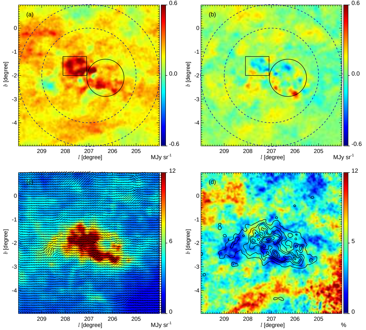
Fig. 3. Planck polarization maps of the Rosette region: (a) Q Stokes parameter; (b) U Stokes parameter. The dashed circles, with radii 2° and 3°, define the region where we estimate the background level, the full circle centred on the star cluster represents the outer radius of the dust shell, r_{\text{out}}^{\text{dust}} = 22 pc, and the rectangle encompasses the brightest part of the Mon OB2 cloud. (c) Intensity map at 353 GHz with the plane-of-the-sky magnetic field orientation shown by headless vectors, obtained by rotating the polarization angle \psi by 90°. The vectors are plotted at every 6', from the average of Q and U within the same distance from the central pixel. (d) Polarization fraction p , with the same intensity contours as in Fig. 2.
