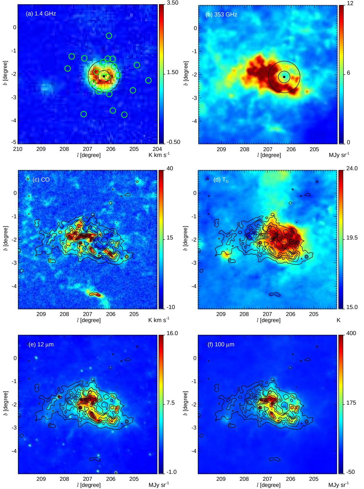
Fig. 2. The Rosette Nebula and its molecular cloud. (a) Integrated RRL emission at 14.4 resolution, showing the radio morphology of the H II region. The green circles, with a diameter equivalent to the beam full width at half maximum (FWHM) of the RRL data, give the position of the 20 RM observations of Savage et al. (2013) used in this work. (b) Planck 353 GHz emission at 6' resolution. The black star in panels (a) and (b) indicates the position of the central star cluster NGC 2244 and the black circles correspond to the inner and outer radii of the H II region, r_{\text{in}}^{\text{H II}} = 7 \text{ pc} and r_{\text{out}}^{\text{H II}} = 19 \text{ pc} , respectively (see Sect. 4.2.2). (c) Planck CO integrated intensity at 5.5' resolution. (d) Dust temperature derived from Planck at 5' resolution. (e) Dust emission as seen by IRAS at 12 \mu\text{m} and at 100 \mu\text{m} (f), at 4' resolution. The contours in panels (c) to (f) show the Planck 353 GHz emission; these are at every 5 % from 15 to 30 %, at every 10 % from 30 to 50 %, and finally at 70 and 90 % of the maximum intensity of 37 \text{MJy sr}^{-1} .
