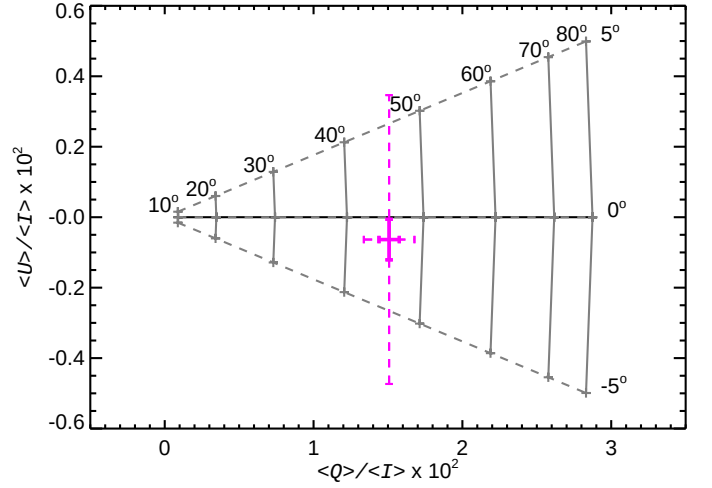
Fig. 7. Comparison between the Planck observations and the model. The ratios \langle Q \rangle / \langle I \rangle and \langle U \rangle / \langle I \rangle derived from the polarization data are given by the magenta point. The statistical and systematic uncertainties are shown by the solid and dashed error bars, respectively. The dashed grey lines show the solutions for \phi_0 = -5^\circ, 0^\circ , and 5^\circ , with \theta_0 varying from 10^\circ to 80^\circ . The solid grey lines indicate how the ratios change with \phi_0 , for a given \theta_0 angle. The model results are calculated here for p_0 = 4\% .
