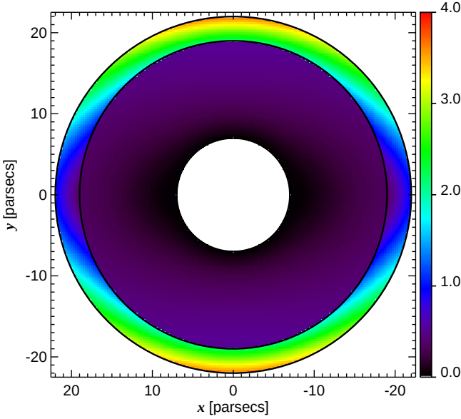
Fig. A.3. Ratio of the field strength B/B_0 for a vertical slice through the centre of the bubble-shell structure ( xy plane). The initial field \mathbf{B}_0 is on the plane of the sky ( \theta_0 = 90^\circ ) and along x ( \phi_0 = 0^\circ ). The three black circles delineate the radii of the Rosette H II and dust shells: r_{\text{in}}^{\text{H II}} = 7 pc; r_{\text{out}}^{\text{H II}} = r_{\text{in}}^{\text{dust}} = 19 pc; and r_{\text{out}}^{\text{dust}} = 22 pc.
