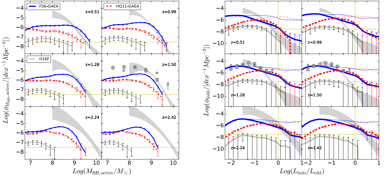
Figure 7. Left-hand panel: Redshift evolution of the mass function of active BHs, defined as sources powering AGNs more luminous than L_{\text{bol}} > 10^{44.6} \text{ erg s}^{-1} . Right-hand panel: Redshift evolution of the probability distribution function of Eddington Ratios. Black, red, and blue lines correspond to GAEA runs as in Fig. 2. Dashed lines refer to the sample of model AGNs more luminous than L_{\text{bol}} > 10^{44.6} \text{ erg s}^{-1} , while solid lines show the distribution for a sample selected using both the bolometric luminosity ( L_{\text{bol}} > 10^{44.6} \text{ erg s}^{-1} ) and BH mass ( M_{\text{BH}} > 10^8 M_{\odot} ) selections. Data are from Kelly & Shen (2013, shaded area) and Schulze et al. (2015, dots with errorbars).
