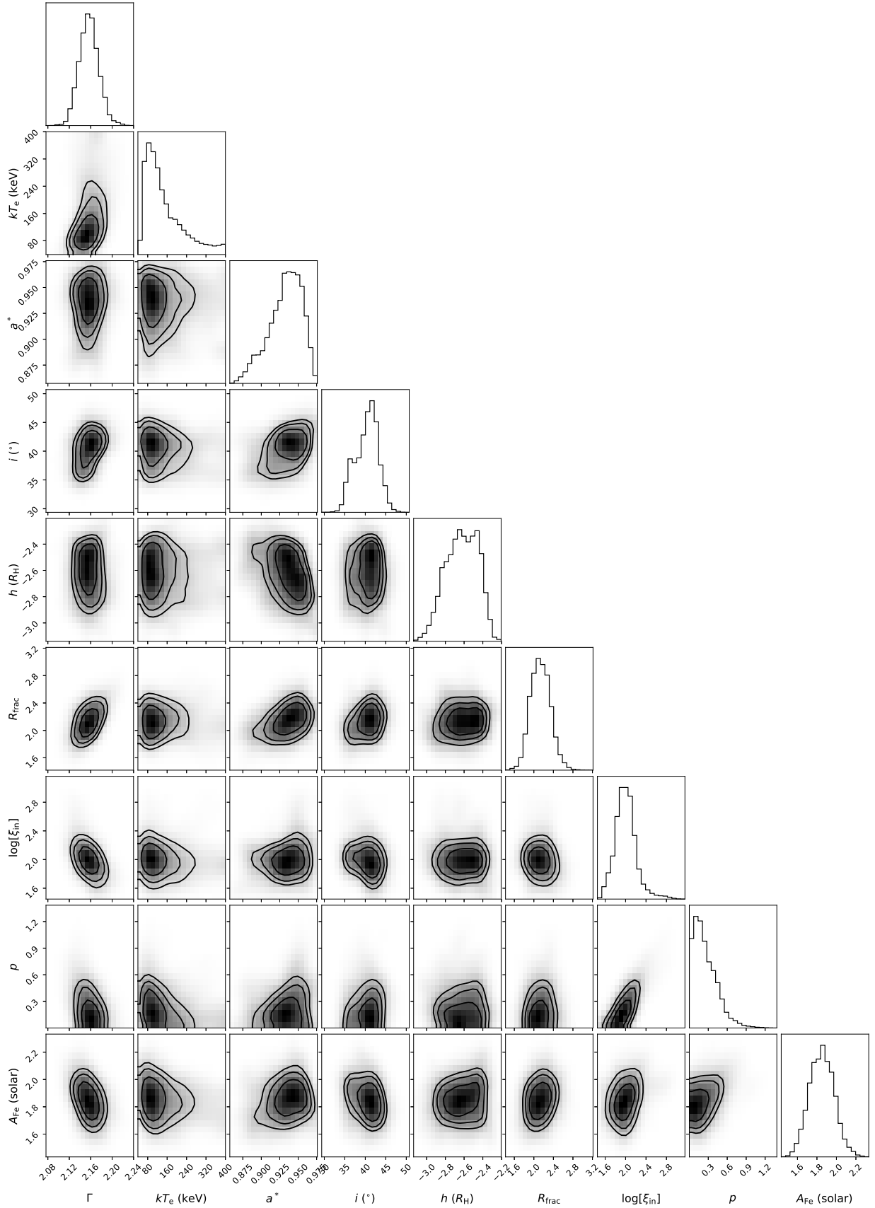
Figure A1. The MCMC results for parameters relating to the intrinsic AGN continuum and the relativistic disc reflection for the data from epoch 1. The plot format follows that of Figure 8.
