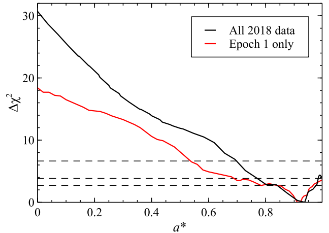
Figure 13. The \Delta\chi^2 confidence contours for the spin of IRAS 09149–6206 based on our spectral modeling of the full 2018 dataset with R_{\text{frac}} computed self-consistently from a^* and h in the lamppost geometry (black; see Section 3.2.2). For comparison, we also show the equivalent contour based on just the coordinated XMM-Newton + NuSTAR data (epoch 1; red, as in Figure 7). The horizontal dotted lines again represent the 90, 95 and 99% confidence levels for a single parameter of interest.
