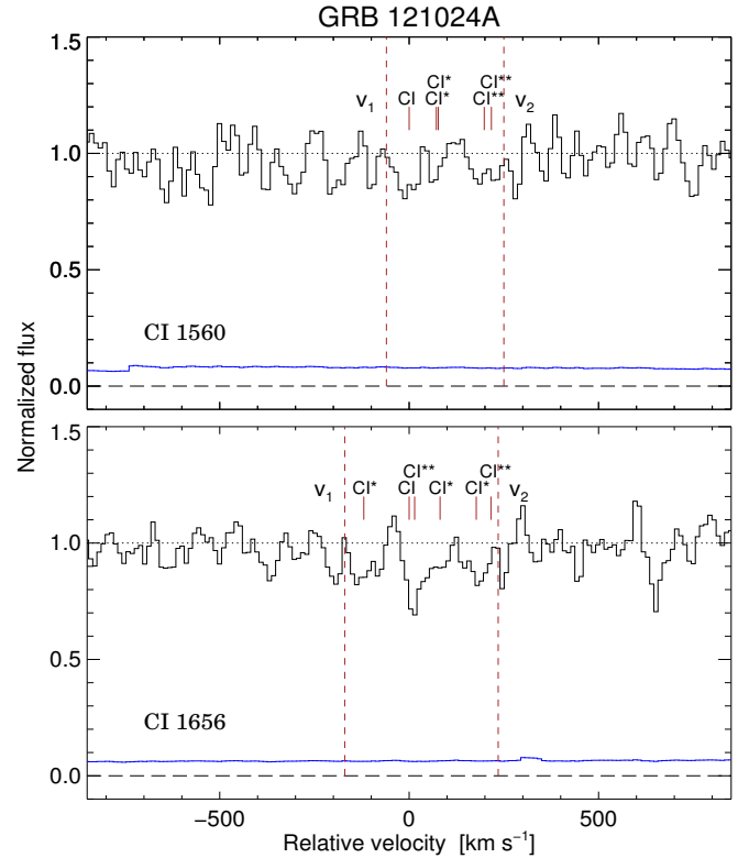
Fig. 3. Same as Fig. 1 but for GRB 121024A, centred on z = 2.3021 . C I is detected below the completeness limit in this system.
