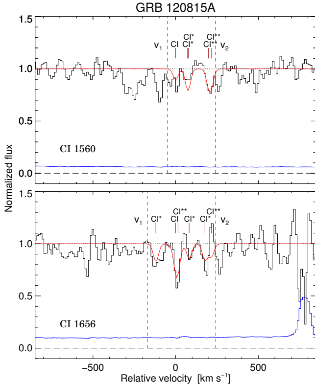
Fig. 2. Same as Fig. 1 but for GRB 120815A, centred on z = 2.3581 . Consistent absorption profiles are also detected in C I \lambda 1277 and C I \lambda 1328. Overplotted in red are the best-fit Voigt profiles. C I is detected below the completeness limit in this system.
