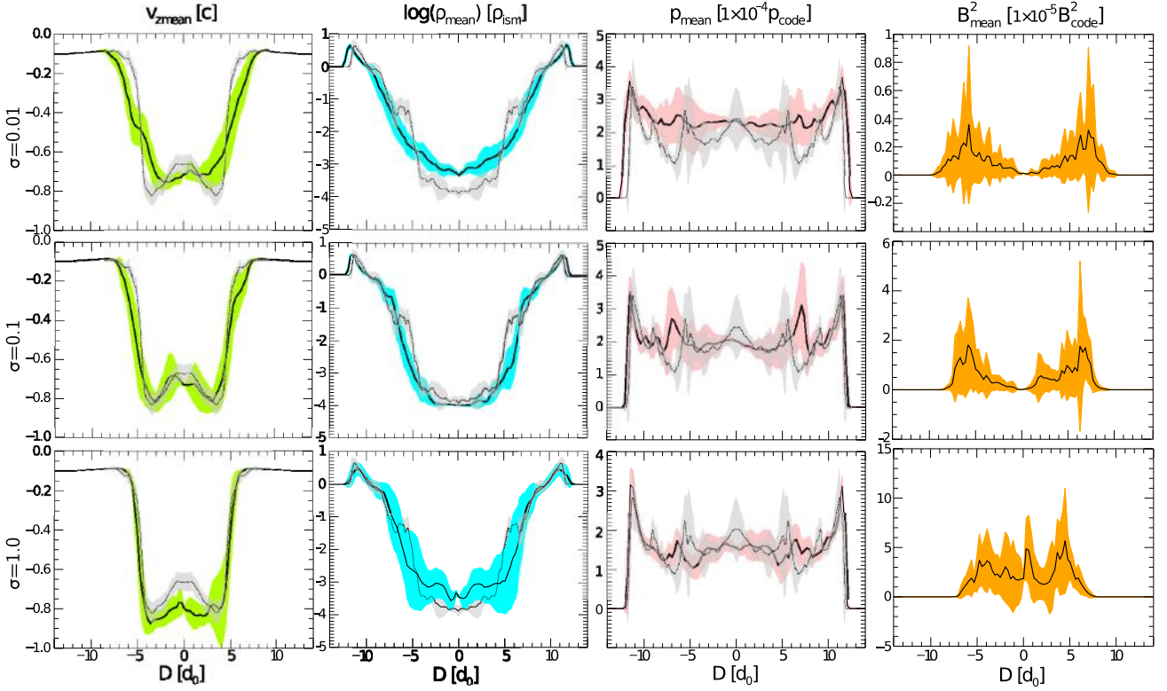
Figure 9. Comparison of the average 1D profiles extracted from different 2D maps at various distances from the pulsar (namely z = -20.0d_0 , z = -20.8d_0 , z = -21.7d_0 ) for run I_{\{0,i\}} . Columns refers to the same variable (from left to right: v_z , \log \rho , p , B^2 ) and rows to the same magnetization (from top to bottom \sigma = 0.01 , \sigma = 0.1 , \sigma = 1.0 ). Black solid lines indicate the computed average trend of each variable and the surrounding coloured area the related standard deviation. The superimposed black dotted line and grey areas are profiles and standard deviations extracted from 2D- H_0 , for comparison. Spatial scales are given in d_0 units. Notice that p is given in 1 \times 10^{-4} p_{\text{code}} units and B^2 in 1 \times 10^{-5} B_{\text{code}}^2 .
