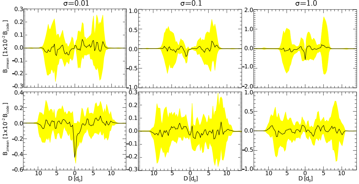
Figure 12. 1D profiles for the B_z component of the magnetic field as function of the distance along the diameter D , in units of d_0 . Upper panel shows plots from runs I_{\{\pi/4,i\}} , bottom for A_{\{\pi/4,i\}} . Solid black lines indicate the average value of B_z and yellow colour areas the corresponding standard deviation. The magnetic field component is here given in 10^{-2} B_{code} units.
