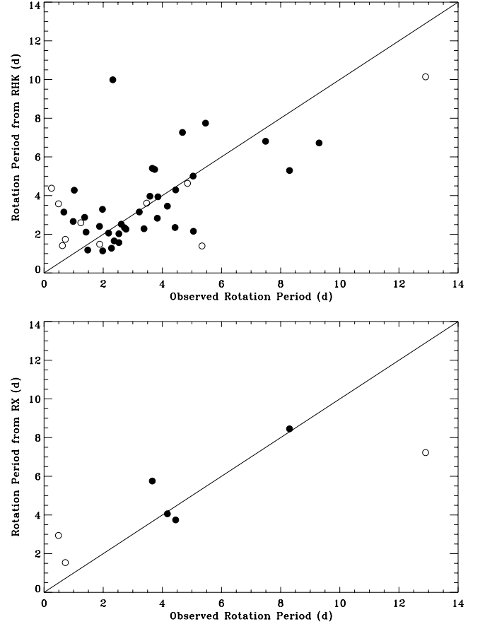
Fig. 7. Observed rotation period vs. the expected rotation period from the value of \log R_{\text{HK}} (upper panel) and R_X (lower panel), as derived by using the Mamajek & Hillenbrand (2008) calibrations. Filled circles represent stars with confirmed or likely rotation period. Empty circles represent stars with uncertain rotation period. The outlier in the upper panel is represented by HIP 79958. As the measured rotation period appears to be robust, the discrepancy may be due to poor sampling of H and K variability or due to calibration issues resulting from the low temperature of the star. See Appendix B for further details.
