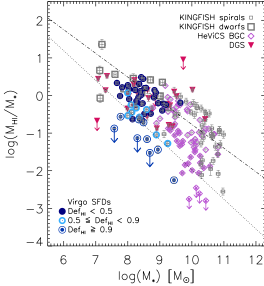
Fig. 5. HI gas fraction ( M_{\text{HI}}/M_* ) as a function of stellar mass. Blue symbols correspond to the Virgo SFDs, with the different shapes indicating the atomic hydrogen content of the galaxies as given by the HI deficiency parameter: HI-normal (filled dots), HI-deficient (rings), highly HI-deficient (ringed dots). Red-purple triangles represent the DGS sample, grey squares show the spiral and dwarf galaxies of the KINGFISH sample, and purple diamonds correspond to the HeViCS BGC. HI-deficient HeViCS BGC galaxies ( \text{Def}_{\text{HI}} \geq 0.5 ) are indicated by a diamond with a cross. Gas-scaling relations from Gavazzi et al. (2013b) are overlaid for normal (dash-dotted line), and highly deficient (dotted line) galaxies.
