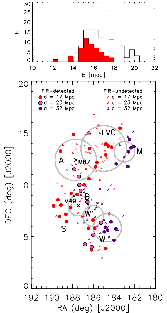
Fig. 1. Upper panel: distribution of apparent B magnitudes of the Virgo Sm, Im, and BCD galaxies in the four HeViCS fields. The red filled histogram shows the galaxies detected by Herschel . The dotted line corresponds to the completeness limit of the VCC catalogue. Lower panel: spatial distribution of the Sm, Im, and BCD galaxies in the four HeViCS fields. Grey circles show the main substructures within the cluster. Filled red, pink, and purple dots indicate FIR detections in at least two Herschel bands at distances of 17, 23, and 32 Mpc, respectively, that will be analysed in this work. Triangles with the same colour codes correspond to FIR non-detections at the three distance ranges.
