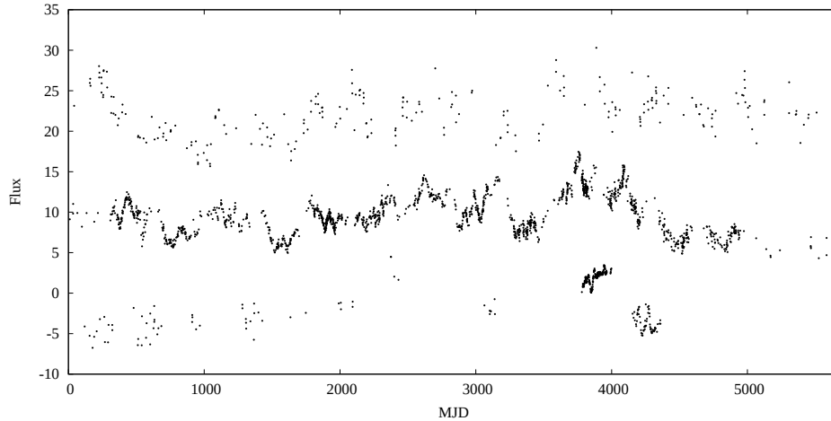
Figure 1. Folded phased diagram of NGC 5548 continuum flux 45 yr long light curve, assuming 5676 days periodicity, here presented to show an example of repeating noisy pattern light curve. Top light curve is pre AGN watch epoch, middle is AGN watch epoch Sergeev et al.(2007), and bottom is post AGN watch epoch constructed from new observations presented in Bon et al.(2016), Lu et al.(2016), Pei et al.(2017).
