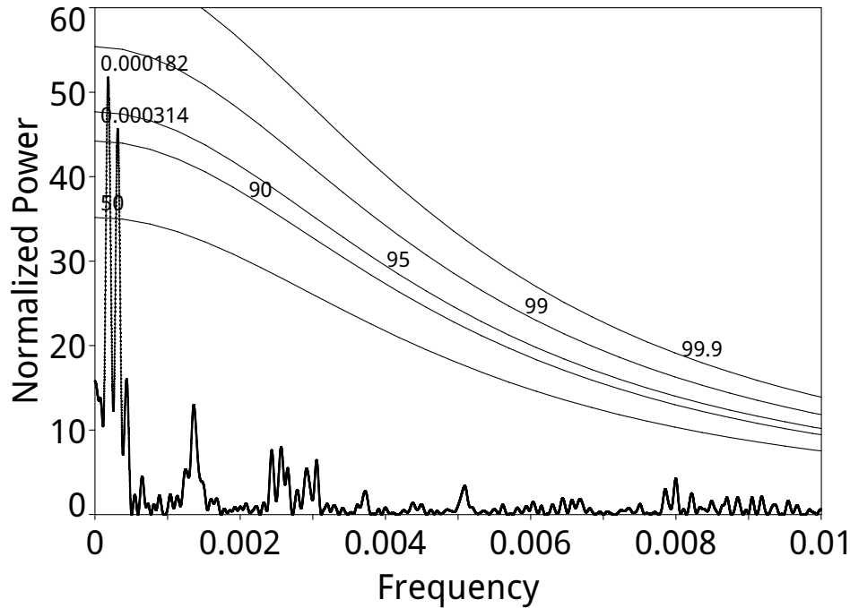
Figure 2. Example of Lomb-Scargle periodogram of NGC 5548 radial velocity curve constructed from the red side broad H\beta half-widths measured at 75% of maximum (see Bon et al. 2016). Red noise background spectrum significance levels are marked.
