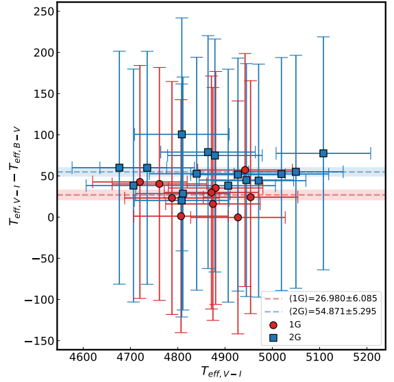
Fig. F.2. Shift in temperatures for our RGB targets when the estimate is carried out with the B - V or the V - I colours. The dashed lines are the average values for the two populations with their respective 1\sigma interval.
