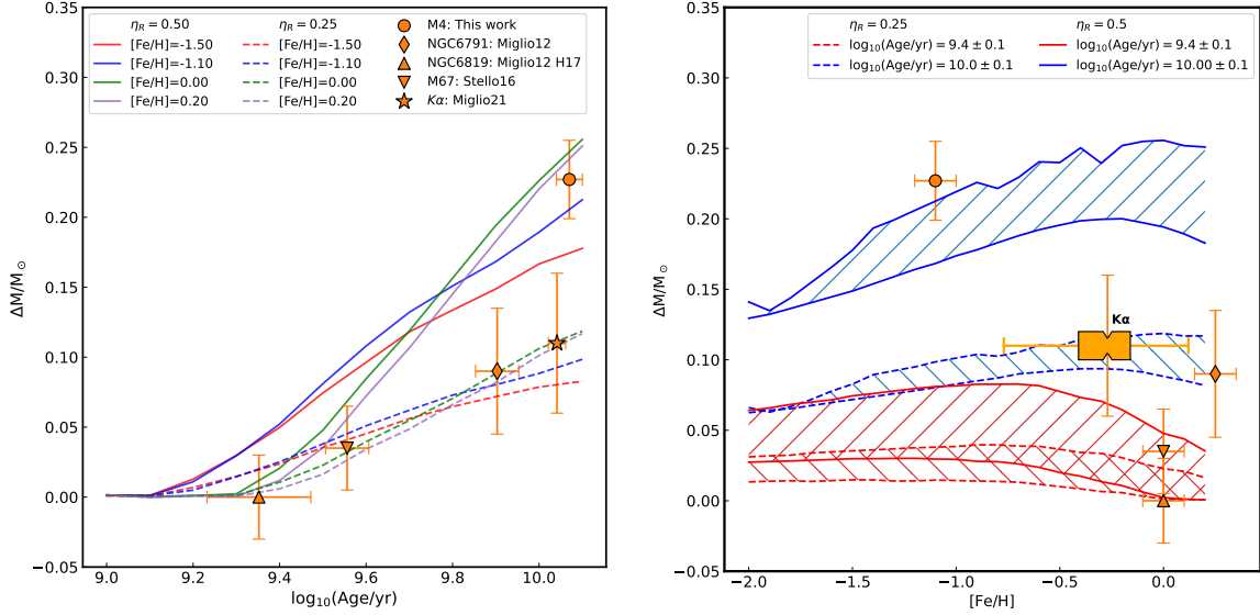
Fig. 4. Mass loss measured using asteroseismic observables for M4, NGC 6791 (Miglio et al. 2012), NGC 6819 (Miglio et al. 2012; Handberg et al. 2017, H17), M67 (Stello et al. 2016), and the \alpha -enhanced stars in the Kepler field ( K\alpha , Miglio et al. 2021) as function of age (left) and metallicity (right). Two sets of models for different (Reimers 1975) mass loss parameter, \eta_R = 0.25, 0.50 , are included for comparison purposes.
