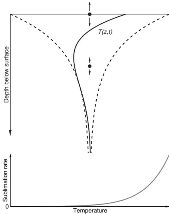
Fig. 7 Schematic illustration of a subsurface temperature profile (solid line = instantaneous, dashed lines = minimum and maximum). Any volatile water molecule has a certain probability to hop up or down. A water molecule on the surface (upper dot) has a different mobility than a molecule at depth (lower dot) where temperature and temperature amplitude are different. In the long term, this leads to a net vertical flux of water molecules. When that flux is downward, this acts as an “ice pump”. The nonlinear dependence of the sublimation rate on temperature is also illustrated (gray line). From Schorghofer and Aharonson (2014)
