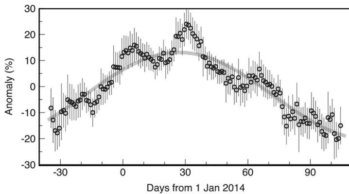
Fig. 13 The deviation of argon exospheric surface density measured from LADEE/NMS (circles with 1- \sigma error bars) from a steady state model based on thermal desorption (gray line). From Hodges and Mahaffy (2016)
