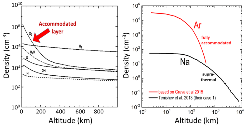
Fig. 2 Left: Estimated average European exospheric densities for selected species from the model of Smyth and Marconi (2006). Sufficiently volatile species like O 2 and H 2 O exhibit a low altitude thermally accommodated layer, but at high altitudes the dominance of supra-thermal (non-accommodated) molecules newly produced/ejected from the surface results in a shallow slope of density versus altitude. Right: Lunar Ar and Na gas densities at sub-solar noon, from the models used by Grava et al. (2015) and Tenishev et al. (2013) to fit LACE Ar and remote Na observations. Na density taken from Tenishev et al. (2013); their case 1 that assumes full Na sticking to the surface. Ar density versus altitude is extracted from the Grava et al. (2015) model. Lunar Ar is fully thermally accommodated resulting in a steep slope versus altitude. Lunar Na is freshly ejected largely by photon-stimulated desorption. Therefore Na is not accommodated, producing a shallow slope
