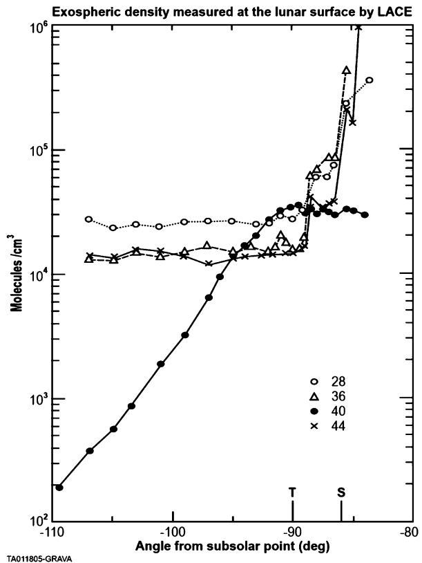
Fig. 14 Surface gas densities measured near lunar sunrise from LACE mass channels 28 ( \text{N}_2 or \text{CO}_2 ), 36 ( ^{36}\text{Ar} ), 40 ( ^{40}\text{Ar} ), and 44 ( \text{CO}_2 ). “T” is the time at which the dawn terminator crossed the landing site, while “S” is the actual sunrise time at the landing site. The ^{40}\text{Ar} density rises as dawn approaches, as exospheric ^{40}\text{Ar} atoms “hop” across the terminator from the dayside and then freeze to the colder night side surface. The lack of a similar pre-dawn rise in \text{CO}_2 is surprising, as \text{CO}_2 is expected to also stick at the Moon’s night side surface temperatures. However the ^{36}\text{Ar} signal is heavily contaminated by instrumental HCl, and all four mass channels rise on the dayside owing to outgassing of hydrocarbon contaminants (Hoffman et al. 1973). Therefore, more measurements are needed to verify LACE’s \text{CO}_2 detection and the contribution of instrumental effects to the data. Figure from Hoffman et al. (1973)
