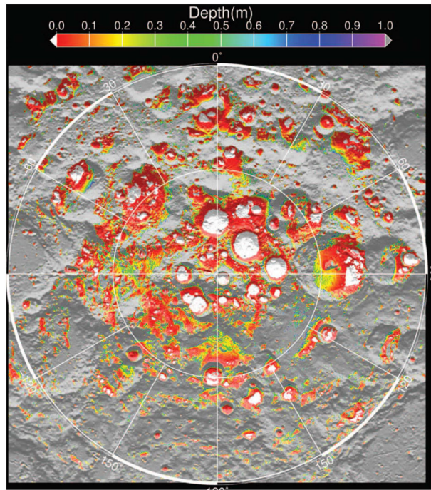
Fig. 10 Near surface ice stability is modeled to be possible over vastly larger areas than strict permanently shadowed regions (white areas). The colored regions represent different depths to reach ice stability in the top 1 meter of regolith. From Paige et al. (2010)
