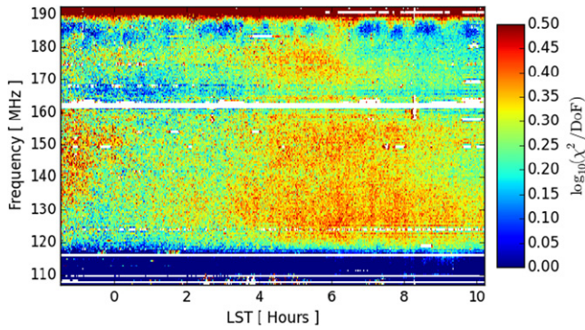
Figure 5. Log of \chi^2 per degree of freedom of all baseline residuals after the application of OMNICAL. The plot comprises observations over one day, with a frequency resolution of 493 kHz and a time resolution of 42.9 s.
