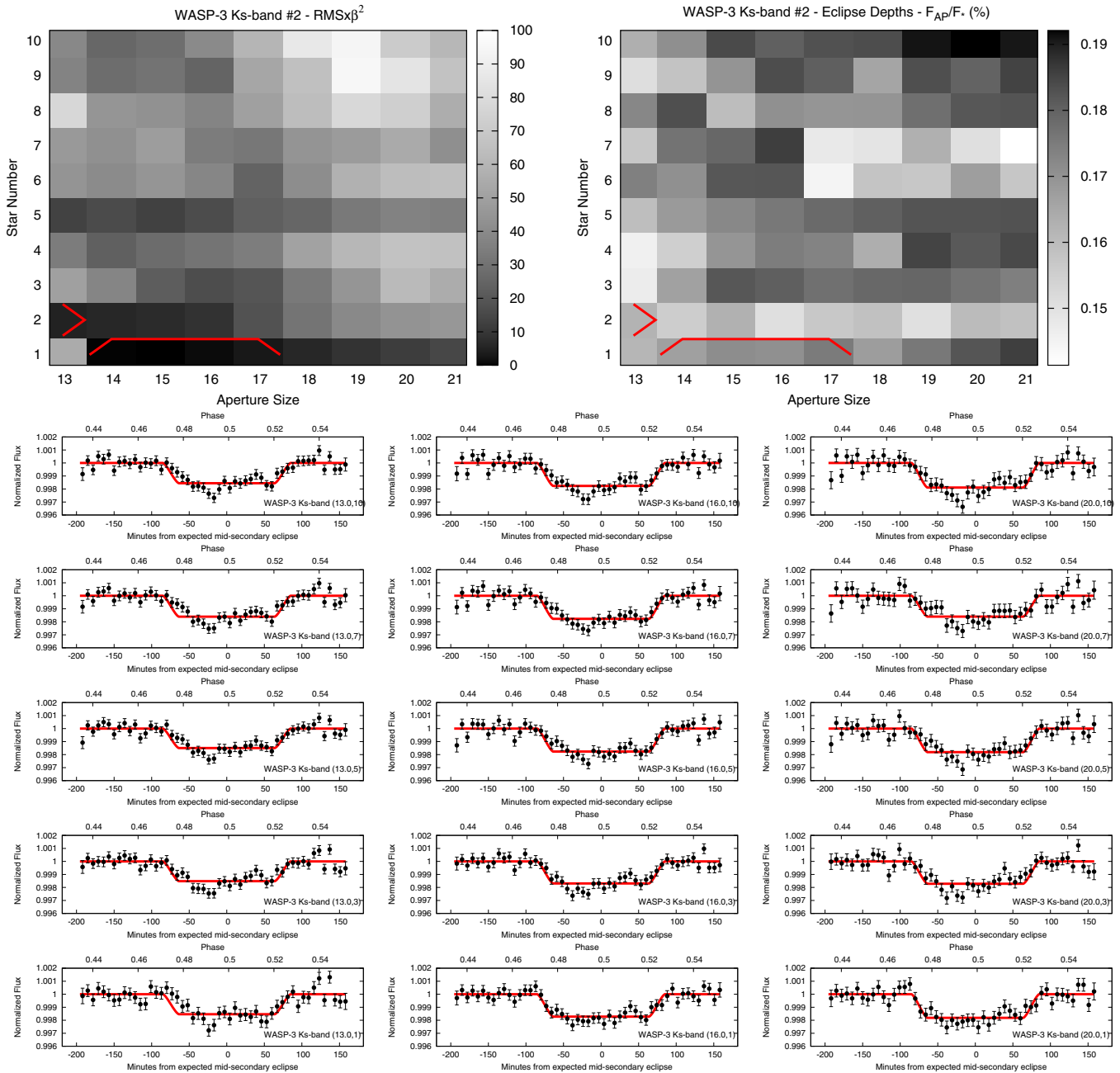
Figure 19. Same as Figure 13 except for our second WASP-3 Ks-band secondary eclipse. The scale of the bottom panels is identical to that of the other WASP-3 Ks-band eclipse (Figure 18). For our second WASP-3 Ks-band eclipse, utilizing more than one reference star introduces correlated noise.
