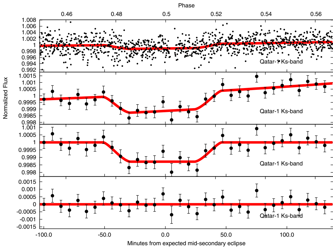
Figure 7. CFHT/WIRCam photometry of the secondary eclipse of Qatar-1b observed in the K_s band on 2012 July 28. The format is otherwise identical to Figure 2.
