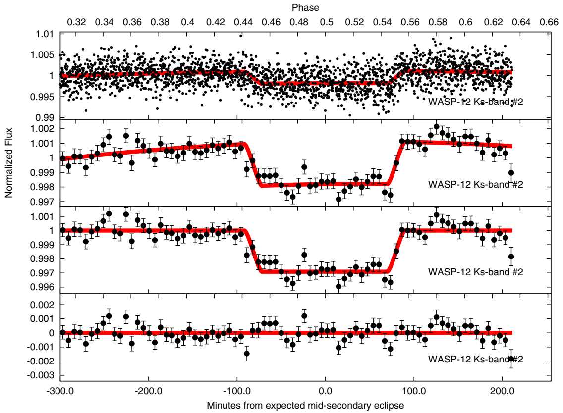
Figure 3. CFHT/WIRCam photometry of the secondary eclipse of WASP-12b observed in the Ks band on 2011 January 14. The format of the figure is otherwise identical to Figure 2, except the data is binned every \sim 6.5 minutes in the bottom three panels.
