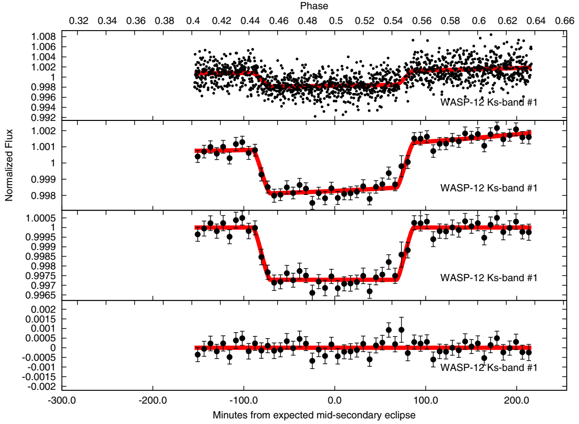
Figure 2. CFHT/WIRCam photometry of the secondary eclipse of WASP-12b observed in the Ks band on 2009 December 28. The top panel shows the unbinned light curve with the best-fit secondary eclipse and background from our MCMC analysis (red line). The second panel shows the light curve with the data binned every \sim 7.0 minutes and again our best-fit eclipse and background. The third panel shows the binned data after the subtraction of the best-fit background, B_f , along with the best-fit eclipse model. The bottom panel shows the binned residuals from the best-fit model.
