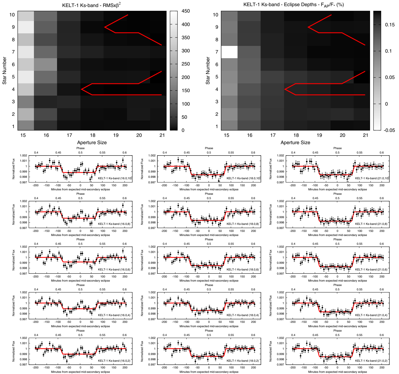
Figure 21. Same as Figure 13 except for our KELT-1 Ks -band secondary eclipse. For our KELT-1 Ks -band eclipse note the obvious correlated noise for the smallest apertures (left panels for the bottom plots).
