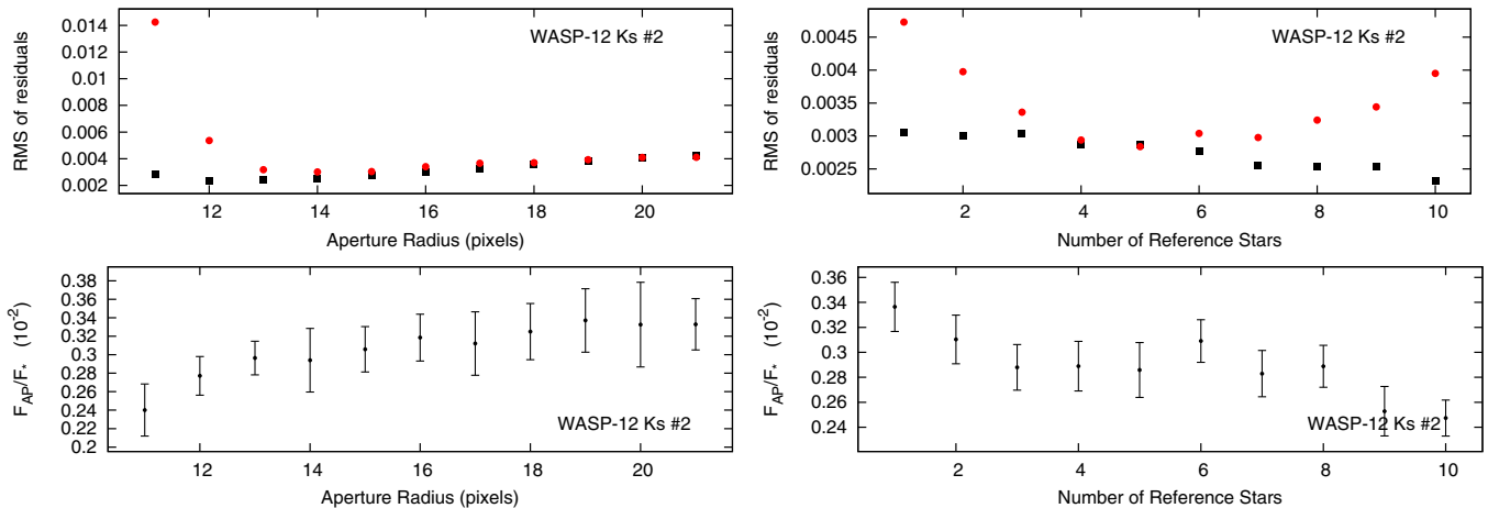
Figure 11. Top panels: the precision of the data for various aperture sizes (left, for a six star reference star ensemble), and for the different number of reference stars for our second WASP-12 Ks -band eclipse (right, for a 15 pixel aperture); the precision of the data is indicated by the rms of the residuals from the best-fit eclipse model (black squares), and the rms of the residuals multiplied by the relevant \beta^2 factor (red circles). Bottom panels: the associated measured MCMC eclipse depths for our second WASP-12 Ks -band eclipse.
