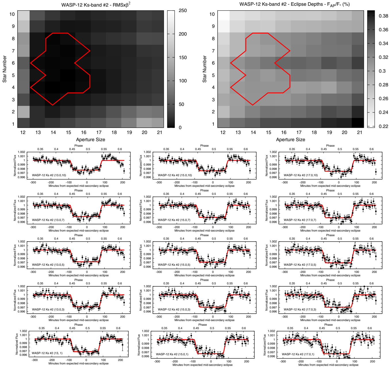
Figure 14. Same as Figure 13 except for our second WASP-12 Ks-band secondary eclipse and the fact that we use a binning time of \sim 6.5 minutes for our bottom panels. The scale of the bottom panels is identical to that of the other WASP-12 Ks-band eclipses (Figures 13 and 15).
