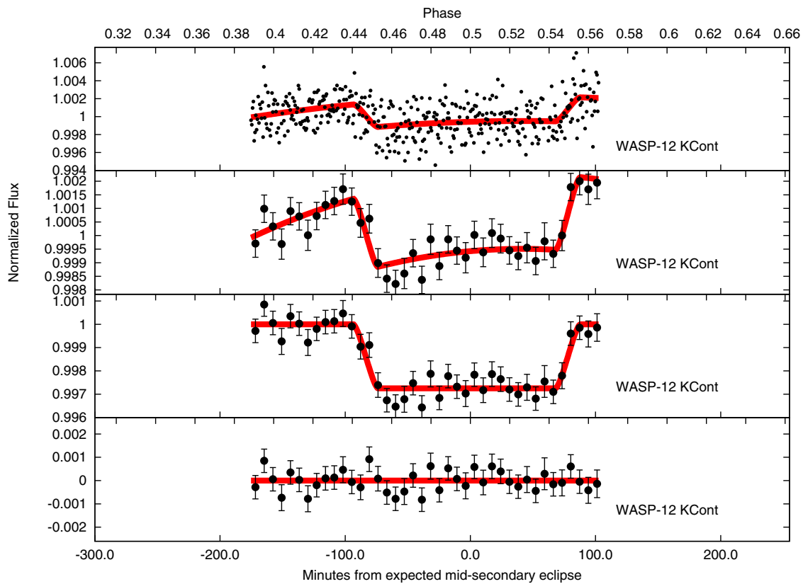
Figure 6. CFHT/WIRCam photometry of the secondary eclipse of WASP-12b observed in the K_{\text{CONT}} band on 2012 January 19. The format is otherwise identical to Figure 2.
