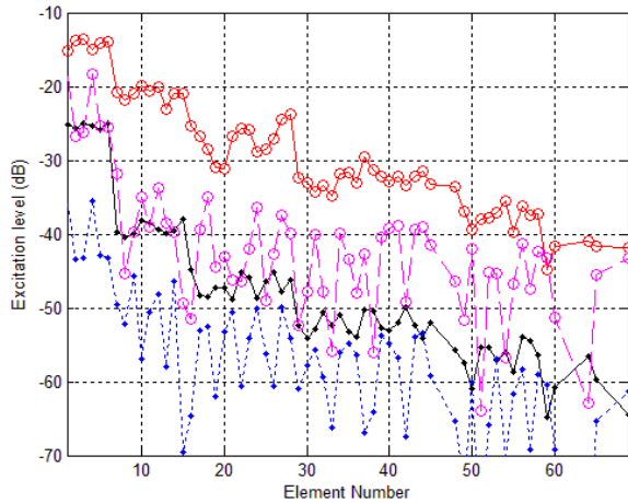
Fig. 6. Magnitude of the quantities \Gamma_L S^{(c)} (co-oriented elements: black solid line with dot markers, cross-oriented elements: blue dashed line with dot markers) and a^{(c)}/a_0 (co-oriented elements: red solid curve with circle markers, cross-oriented elements: magenta dashed line with circle markers) for the LBA elements at 57 MHz with the central element (#0) excited.
