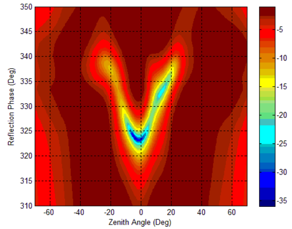
Fig. 8. E-plane pattern cuts (dB) of the LBA central element LEEP at 57 MHz for different values of the amplifier reflection coefficient phase \angle \Gamma_L .
