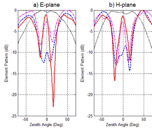
Fig. 7. LEEP principal cuts for the LBA central element at 57 MHz, computed by loading an increasing number of adjacent elements (4): 0 (i.e. unloaded EEP, dotted black curves), 6 (dashed blue curve), 15 (magenta dash-dotted curve) and 45 (solid red curve)
