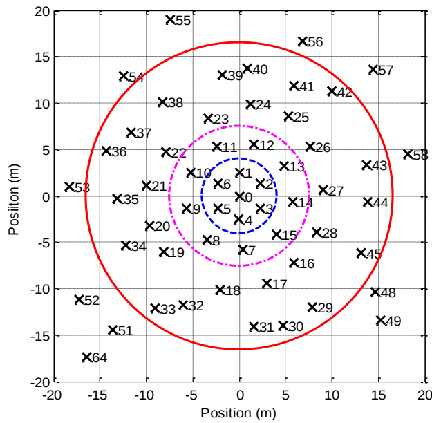
Fig. 5. Distribution of the inner elements of a LOFAR LBA station. The dashed-blue, dash-dotted magenta and the solid red circles identify those elements for which a^{(c)}/a_0 (central one excited) is higher than -15 dB, -25 dB and -35 dB, respectively, at 57 MHz.
