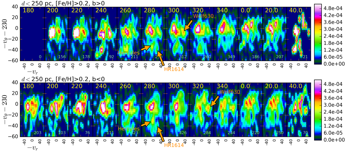
Figure 10. Velocity distributions in uv similar to those shown in Figure 6a for high metallicity stars, but restricted to positive (top panel) and negative (bottom panel) galactic latitudes.
