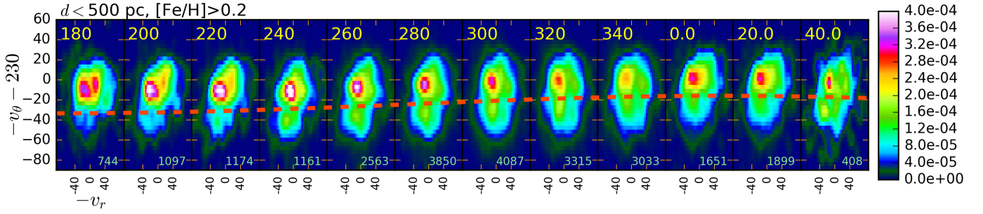
Figure 4. The uv velocity distributions of stars with distances d < 500 pc and [\text{Fe}/\text{H}] > 0.2 as a function of galactic longitude. The orange line (computed with equation 3) corresponds to a gap angular momentum value of L_{\text{gap}} = 1640 \text{ km s}^{-1} \text{ kpc} . The line curves because the galactocentric radius of each neighborhood depends on the viewed longitude. The line suggests that the gap between the Hercules stream and circular orbits is set by a particular angular momentum value, as would be expected with a bar resonant model.
