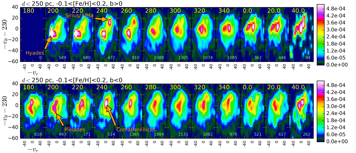
Figure 11. Velocity distributions in uv similar to those shown in Figure 6b for near solar metallicity stars, but restricted to positive (top panel) and negative (bottom panel) galactic latitudes.
