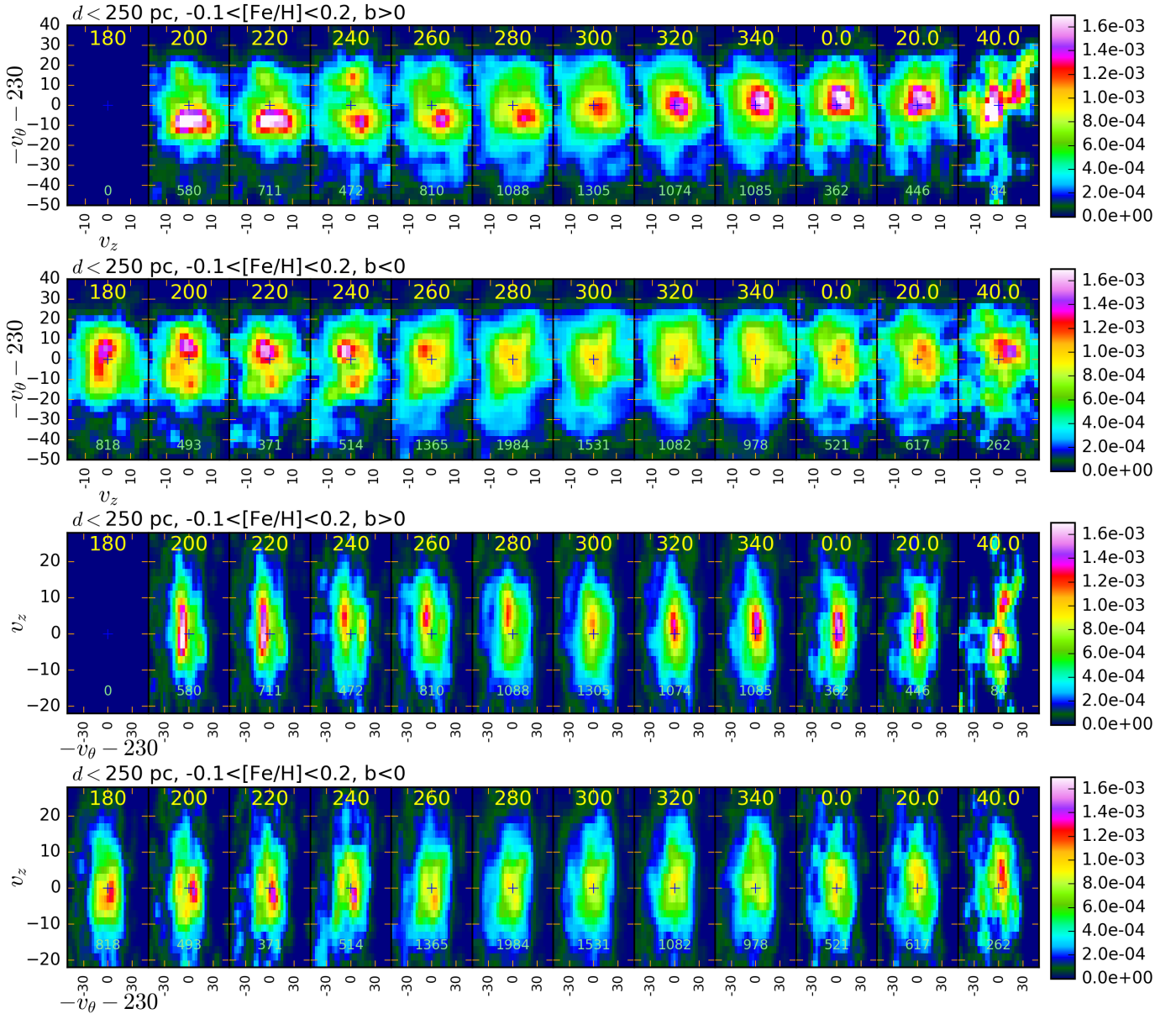
Figure 14. Velocity distributions in v, w for near solar metallicity stars. The x-axes in the top and second from top panels are v and y-axes are w . The third from top and bottom panels are reversed with x-axes w and y-axes v . The top and third from top panels show stars in the northern Galactic hemisphere (latitude b > 0 ) whereas the second from top and bottom panels show stars in the southern Galactic hemisphere.
