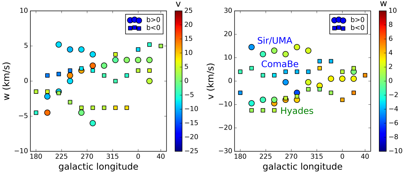
Figure 15. Peaks seen in the d > 250 pc (v, w) velocity distributions of near solar metallicity stars in Figures 14 have w = v_z velocity component plotted as a function of galactic longitude in the left panel. The colour of the points depends on the v velocity (with v = -v_\theta - 230 \text{ km s}^{-1} , as before). In the right panel, the peak v velocity is plotted as a function of galactic longitude and with colour set by the w velocity. Sirius/UMa, Coma Berenices, and Hyades, streams or moving groups are most easily identified in the panel on the right where they are labelled. This Figure is similar to Figure 9 except round points show the northern Galactic hemisphere (galactic latitude b > 0 ) and square points show the southern Galactic hemisphere. The Coma Berenices group is seen in the southern Galactic hemisphere whereas the Sirius/UMa group is seen in the northern Galactic hemisphere. The peak w velocities of each group varies as a function of galactic longitude and Galactic hemisphere. Smooth variations in w with longitude are most easily seen in the right panel.
