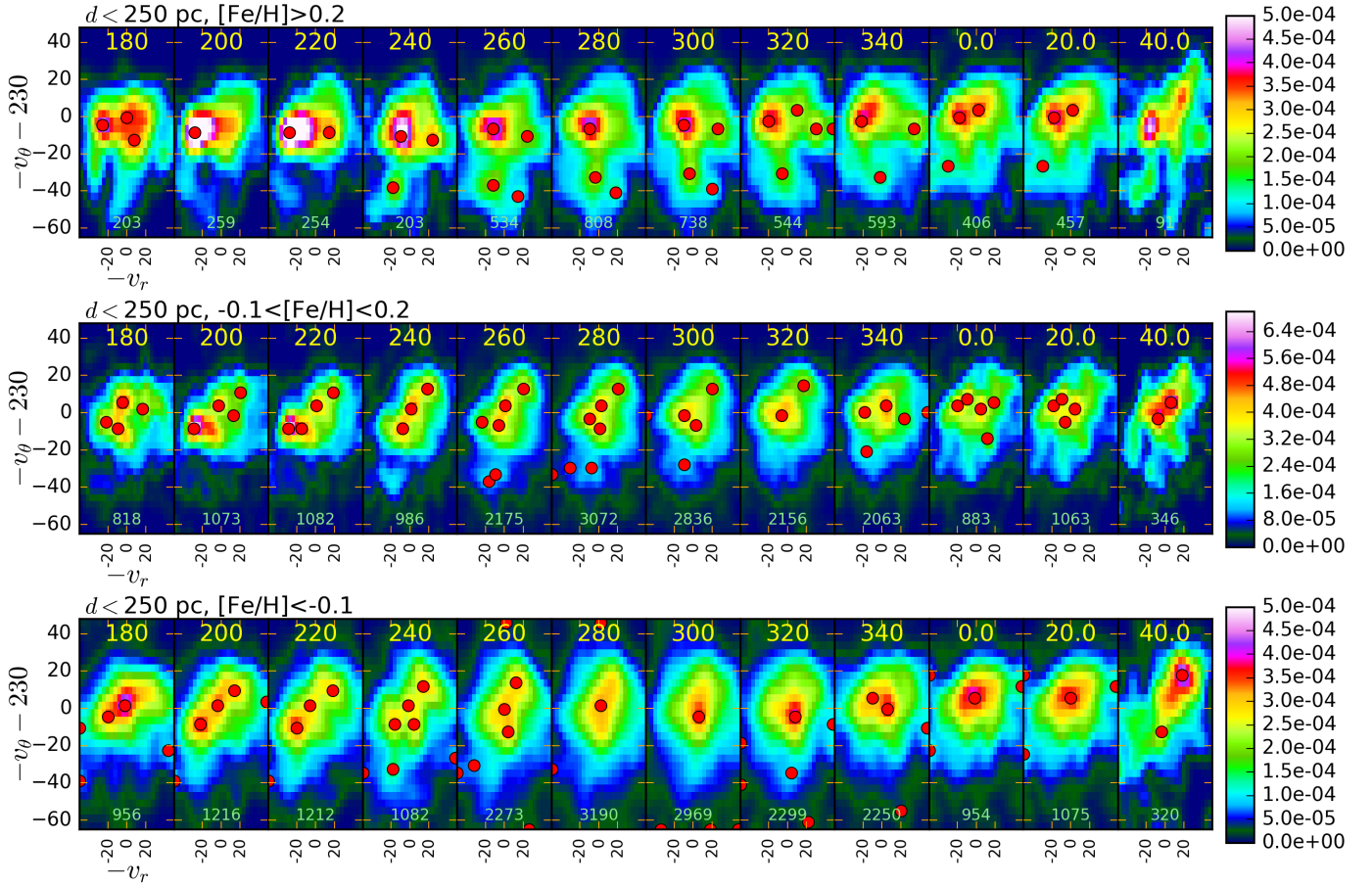
Figure 7. Peaks are found in the uv velocity distributions of nearby stars that are shown in Figure 6. Red dots show the (u, v) velocities of the peaks and they are plotted on top of the velocity distributions.
