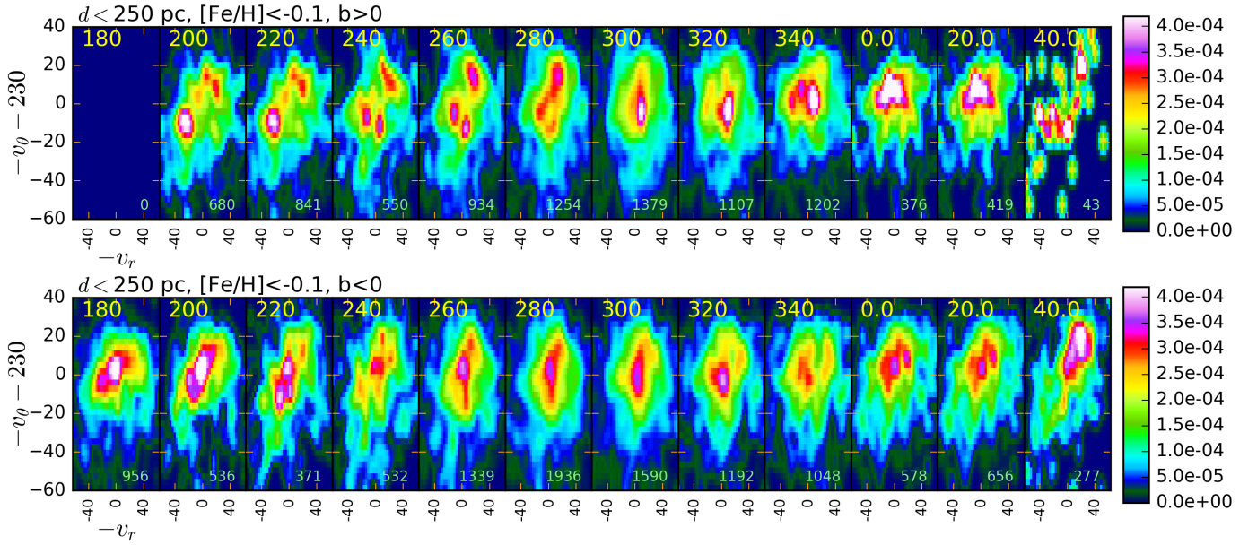
Figure 12. Velocity distributions in uv similar to those shown in Figure 6c for low metallicity stars, but restricted to positive (top panel) and negative (bottom panel) Galactic latitudes. The velocity distributions of low metallicity stars are the most sensitive to Galactic hemisphere, with Coma Berenices moving group preferentially seen in the southern Galactic hemisphere and Hyades and Sirius/UMa groups preferentially seen in the northern Galactic hemisphere.
