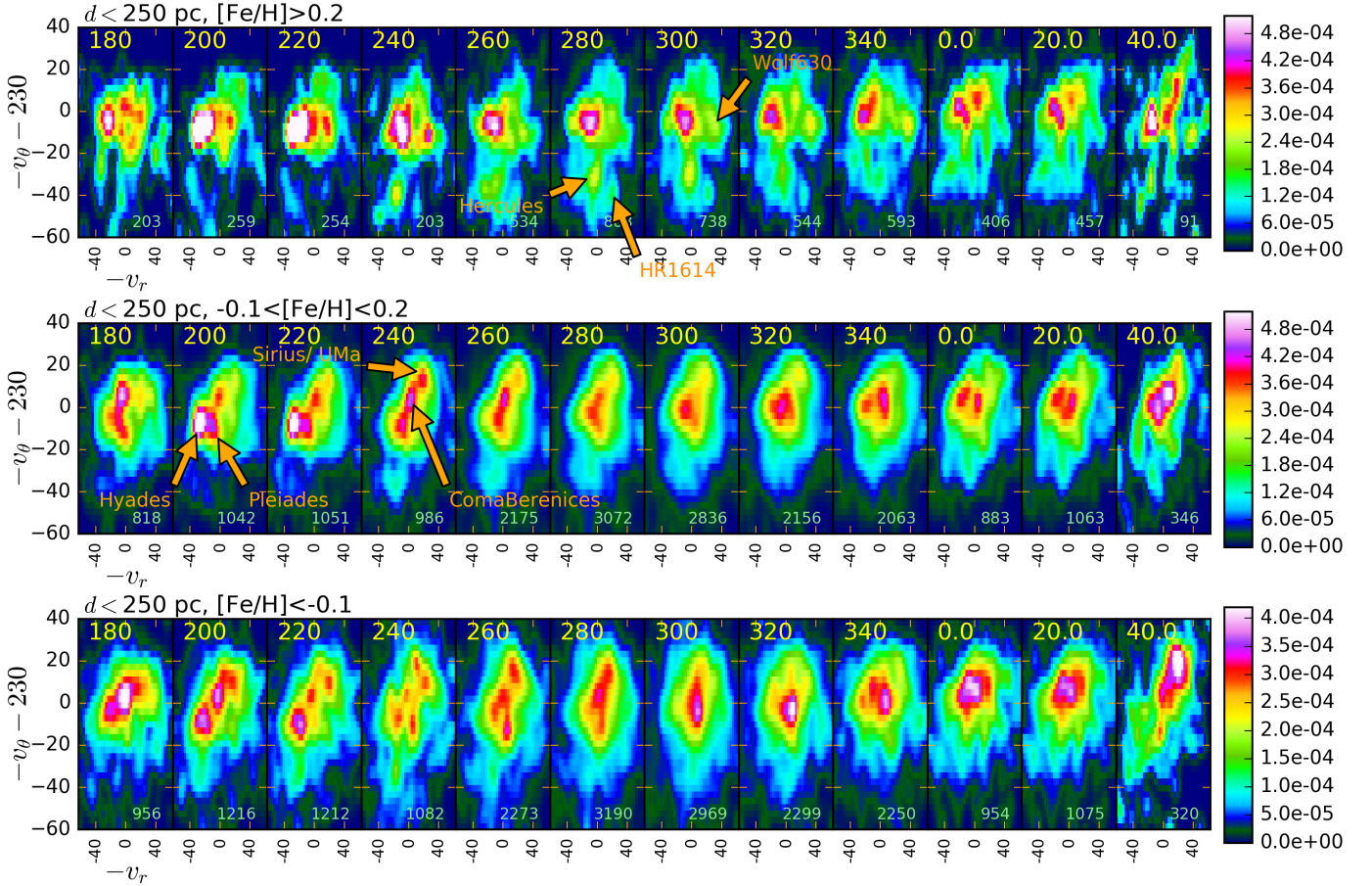
Figure 6. Velocity distributions in uv similar to those in Figure 1 but for nearer stars with distances d < 250 pc. a) For metal rich stars with [\text{Fe}/\text{H}] > 0.2 . b) For near solar metallicity stars -0.1 < [\text{Fe}/\text{H}] < 0.2 . c) For metal poor stars with [\text{Fe}/\text{H}] < -0.1 .
