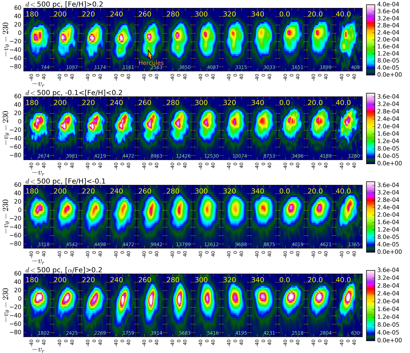
Figure 1. Histograms showing uv velocity distributions constructed of stars viewed at different galactic longitudes. The x-axes show the radial velocities u = -v_r of each bin in \text{km s}^{-1} . The y axes show the tangential velocities v = -v_\theta - 230 \text{ km s}^{-1} of each bin in \text{km s}^{-1} . The histograms only contain nearby stars with distances d < 500 pc. The central galactic longitude for each histogram is the yellow number on the top of each histogram and the number of stars used to construct the histogram shown on the bottom. Each histogram is created using stars within 20^\circ of the central galactic longitude. Each row of histograms is for stars within a different metallicity range. From top panel to bottom panel a) [\text{Fe}/\text{H}] > 0.2 . b) -0.1 < [\text{Fe}/\text{H}] < 0.2 . c) [\text{Fe}/\text{H}] < -0.1 . d) [\alpha/\text{Fe}] > 0.2 .
