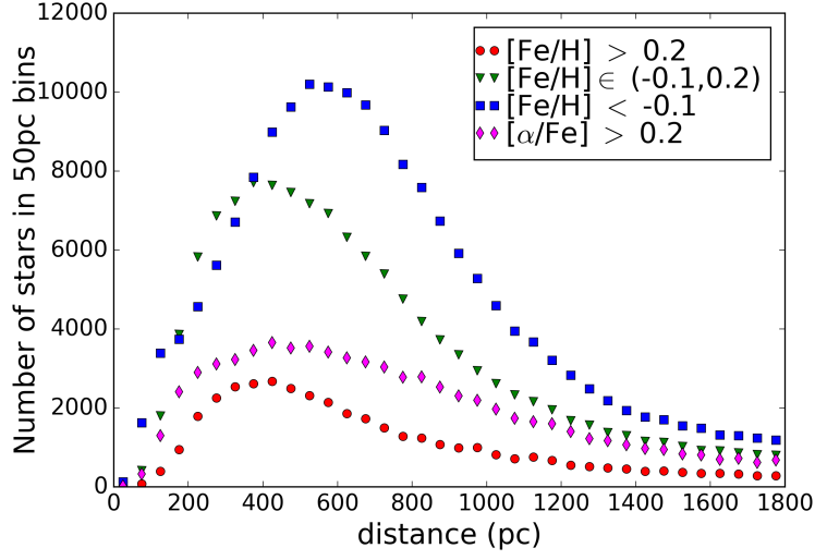
Figure B1. The distribution of distances for the 4 sets of stars used to construct velocity distributions shown in Figures 1– 6.
