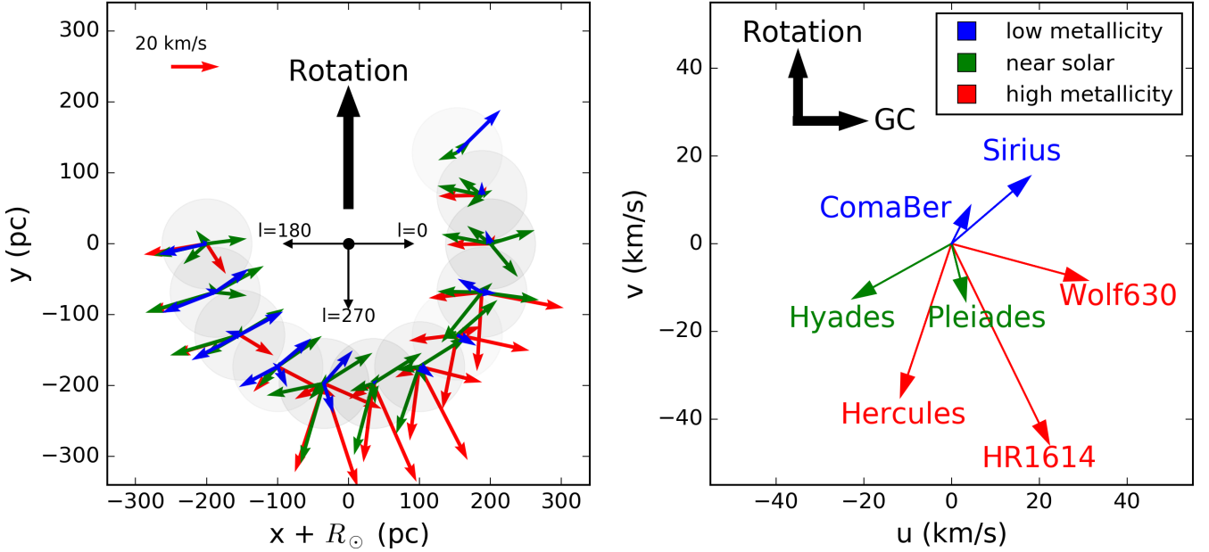
Figure 8. a) Left panel. Peaks seen in the d < 250 pc uv velocity distributions of Figures 6 and 7 are drawn as a function of position in the Galaxy. The x, y axis coordinates are centered about the Sun with positive x toward the Galactic centre and positive y in the direction of rotation. Green arrows show the velocity vectors for peaks in the velocity distribution for solar metallicity stars. Blue arrows are for peaks in the lower metallicity set ( [\text{Fe}/\text{H}] < -0.1 ) and red arrows are for peaks in the higher metallicity set ( [\text{Fe}/\text{H}] > 0.2 ). Coloured arrows are shown for the peaks we identified in Figures 7. Arrow length depends on the u, v velocity vector length. The red arrow on the upper left shows a velocity vector of length 20 \text{ km s}^{-1} . Coloured arrows pointing to the right correspond to motions toward the Galactic centre and arrows pointing upward correspond to motion faster than Galactic rotation. Neighbourhoods are shown as grey filled circles at a distance of 200 pc from the Sun and at galactic longitudes ranging from \ell = 180^\circ (on the left) to 40^\circ on the upper right. Each grey circle represent the location of stars that we see in a particular direction. The smaller black arrows in the centre show the directions of the different galactic longitudes. b) Right panel. The illustration shows the directions of velocity peaks and we have labelled them with the names of moving groups or streams. On this panel thick black arrows show the direction of rotation and the direction of the Galactic centre.
