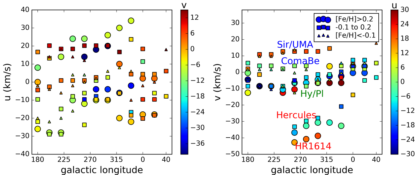
Figure 9. Peaks seen in the d > 250 pc uv velocity distributions of Figures 6 and 7 have u = -v_r velocity component plotted as a function of galactic longitude in the left panel. The colour of the points depends on the v velocity (with v = -v_\theta - 230 \text{ km s}^{-1} as before) and with numbers on the colourbar in \text{km s}^{-1} . In the right panel, the peak v velocity is plotted as a function of galactic longitude and with colour set by the u velocity. In both panels, small triangles are for peaks in the lower metallicity set of histograms ( [\text{Fe}/\text{H}] < -0.1 ), squares are for near solar metallicities ( -0.1 < [\text{Fe}/\text{H}] < 0.2 ) and large circles are for peaks in the higher metallicity set ( [\text{Fe}/\text{H}] > 0.2 ). Sirius/UMa, Coma Berenices, Hyades/Pleiades, Hercules and HR1614 streams or moving groups are most easily identified in the panel on the right where they are labelled. The peak v velocities of each group varies as a function of galactic longitude, with v increasing with increasing longitude over the range (in galactic longitude) where the group is distinctly seen in the local velocity distribution. The Wolf 630 group can be seen on the right panel as red circles in the same region as Hyades and Pleiades. The Hercules stream (with negative u ) and the HR1614 group (with positive u ) can be seen in the left panel as blue circles near galactic longitude \ell = 270^\circ .
