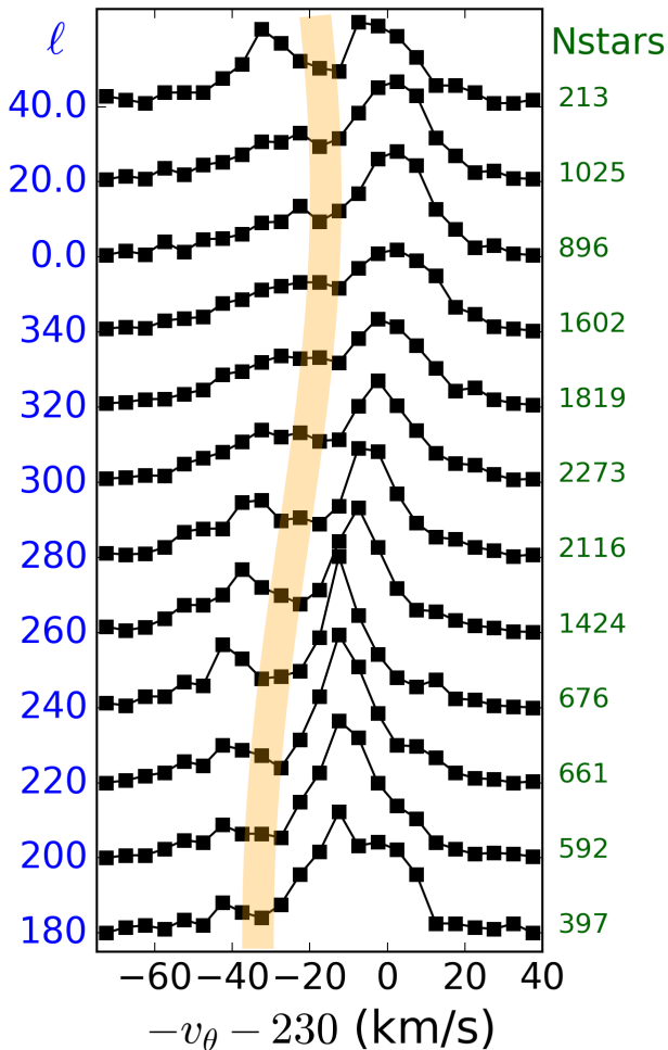
Figure 5. Normalized tangential velocity distributions are shown for stars at each galactic longitude given in blue on the left axis. The numbers of stars in each histogram is shown on the right axis. The vertical range is not shown on either axis. These distributions are similar to that shown in Figure 2 except they are for stars at different galactic longitudes. The thick orange line is computed with equation 3 and corresponds to a gap angular momentum value of L_{gap} = 1640 \text{ km s}^{-1} \text{ kpc} . The Hercules stream forms the peaks at around v \sim -40 \text{ km s}^{-1} that are prominent near galactic longitude \ell = 270^\circ .
